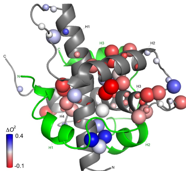
Figure 8. Changes in order parameters (both \Delta O_{\text{NH}}^2 and \Delta O_{\text{axis}}^2 ) for TAZ1 upon binding to CTAD-HIF-1 \alpha are color-coded using a red-white-blue gradient. Large spheres represent the methyl groups and the smaller spheres represent the backbone amide groups. The backbone of TAZ1 is shown in grey, and CTAD-HIF-1 \alpha in green.
