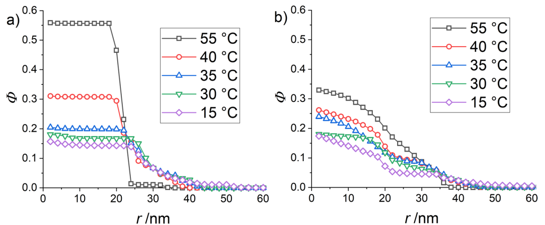
Figure 5. (a) Density profiles of the H-pNIPMAM-core with a CCC of 10 mol% in D 2 O (data adapted from Cors et al. 35 (b) Density profiles of the core monomers of the H-pNIPMAM-core D7-pNIPMAM-shell system with the same core as in (a) and an index-matched shell (CCC = 1.9 mol%).
