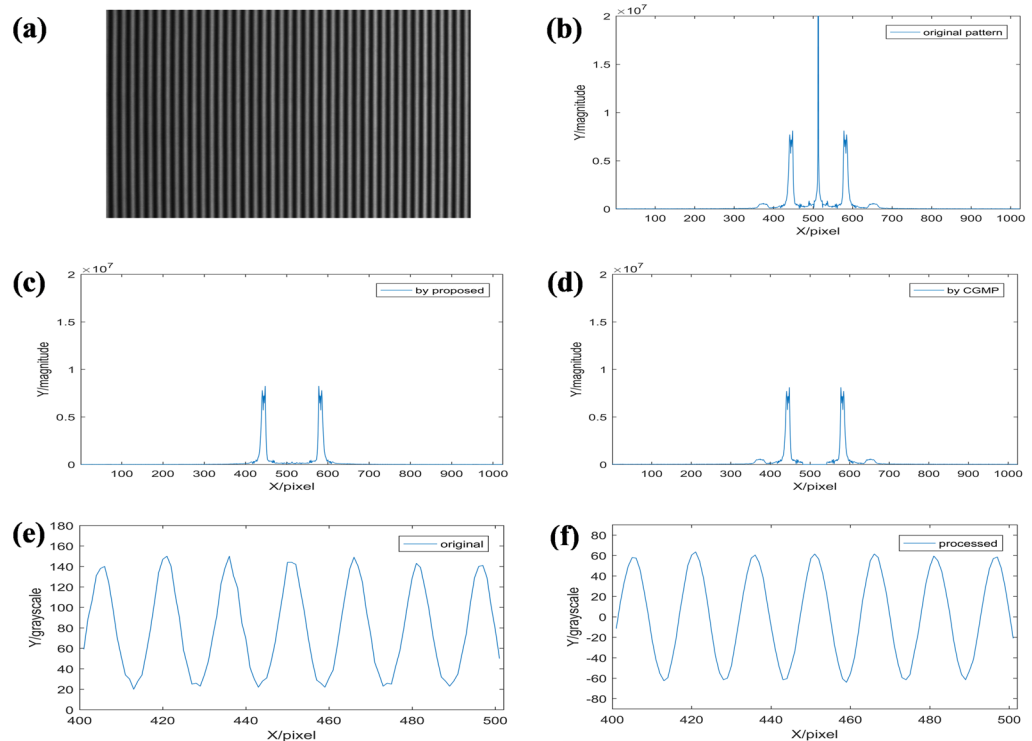
Figure 4. The spectrum analysis: (a) the original fringe pattern; (b) the frequency spectrum of (a); (c) the fundamental frequency component obtained by HCGMP; (d) the fundamental frequency component obtained by CGMP; (e) the cutaway view of (a) in the 400–500 pixel; (f) the corresponding cutaway view of the fringe pattern after background light elimination by HCGMP.
