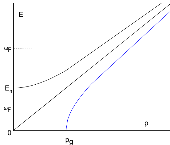
Figure 1. Possible dispersion relations and dependencies of energy E on momentum p . Top curve shows the dispersion relation for a massive particle. Middle curve shows gapless dispersion relation for a massless particle (photon) or a phonon in solids. Bottom curve shows the dispersion relation (3) with the gap in k -space, illustrating the results of ref. 8 . Two values of \omega_F = \frac{1}{\tau} in relation to the energy gap E_g are shown.
