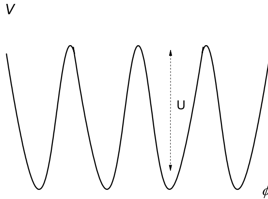
Figure 2. Schematic illustration of an interaction potential.
