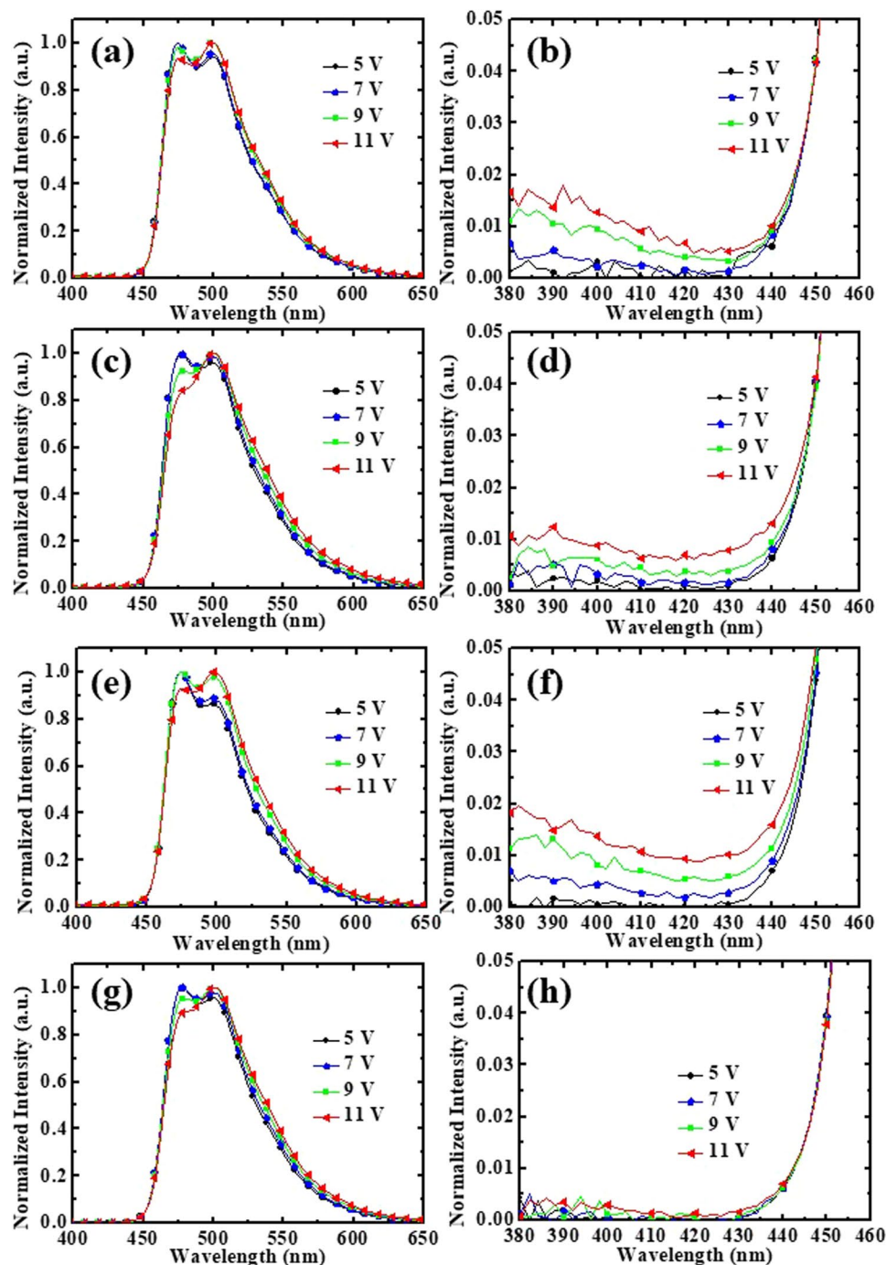
Figure 5. EL spectra at different driving voltages for BPOLEDs with different hosts: (a) mCP, (c) TAZ, (e) mCP:TAZ, and (g) 2CbzTAZ. (b), (d), (f), and (h) are zoomed-in spectra at short wavelength region (380–460 nm) of (a), (c), (e), and (g), respectively.
