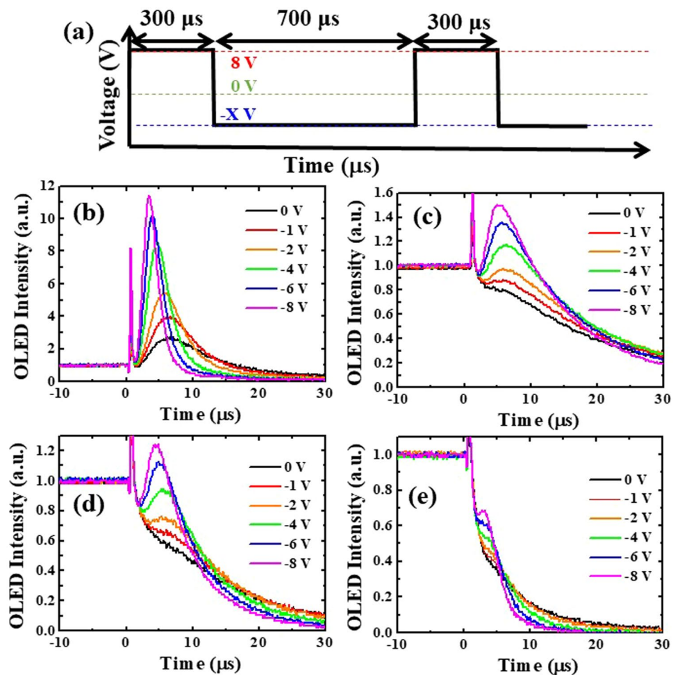
Figure 7. (a) Schematic diagram of waveforms with different reverse biases during off period. Transient luminescence of BPOLEDs with (b) mCP, (c) TAZ, (d) mCP:TAZ, and (e) 2CbzTAZ when the electrical pulse was turned off under different driving waveforms.
