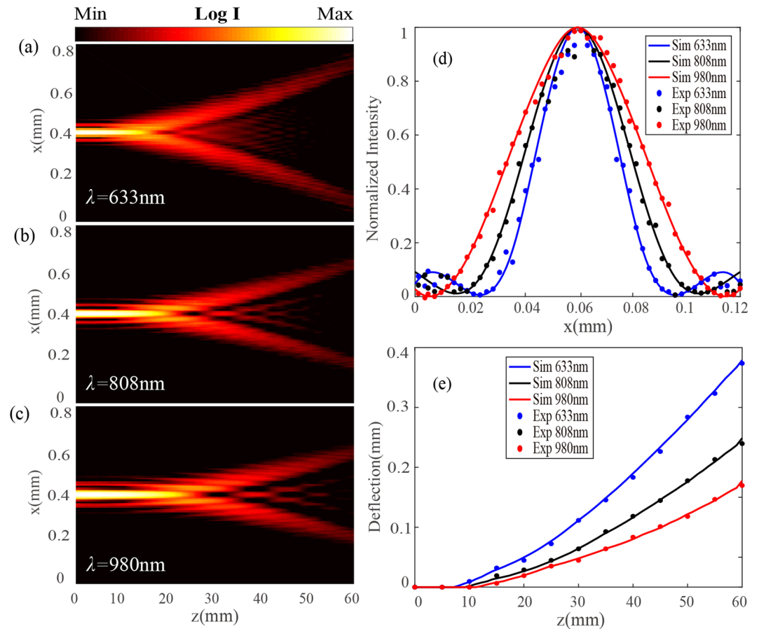
Figure 5. (a–c) Calculated optical intensity profiles in x-z plane for the cusp beams with m = 4 at 633 nm, 808 nm, 980 nm. (d) Calculated and measured transverse intensity distribution at z = 0 plane. (e) Calculated and measured beam deflection along the curved cusp lobes during the propagation.
