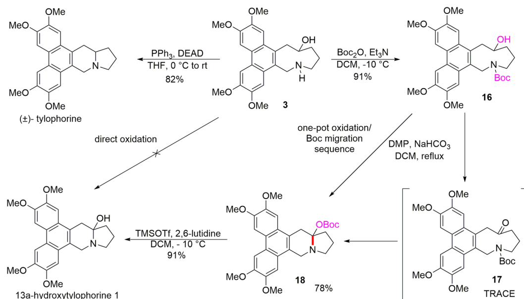
Figure 5. Syntheses of (±)-tylophorine and 13a-hydroxytylophorine (1).
