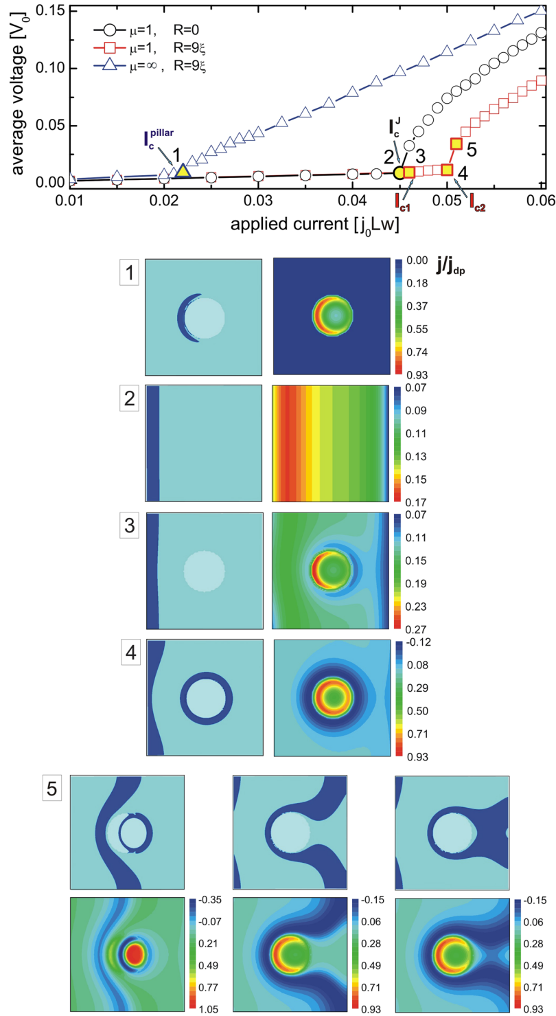
Figure 5. Current-voltage characteristics and current distribution related to vortex behavior. Main panel: Current-voltage ( I - V ) characteristics of the sample with L = w = 50\xi , d = 5\xi , \delta = 1\xi , junction parameters \mu = 1 , \zeta = 1 , and applied magnetic field H = 0.01H_{c2} : (i) with a pillar of radius R = 9\xi and no Josephson coupling ( \mu = \infty , blue triangles), (ii) with no pillar but with Josephson coupling (black circles), (iii) with both Josephson coupling and a pillar of radius R = 9\xi (red squares, closely corresponding to the case of Fig. 2). Labeling of the characteristic threshold currents in the main panel follows the detailed discussion in the text. Panels (1–4) Represent the isosurface plots of the Cooper-pair density and the corresponding current density distribution in the stationary states found at the applied currents indicated by yellow filled symbols in the main panel. Panel (5) same as panels 1–4, but shows the temporal sequence of non-equilibrium states upon onset of the resistive state in case (iii). Note: in panels (1–5) the current density is normalized by the depairing current density j_{dp} = 0.38j_0 .
