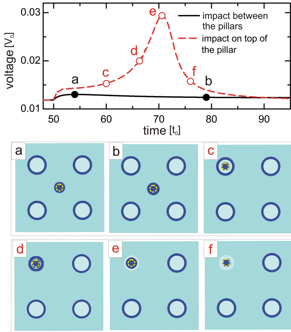
Figure 7. Response of the Josephson loop to a focused laser beam. Voltage-time response of the sample of Fig. 2, when the laser impact (at t_l = 50t_0 ) occurs between the pillars (solid black curve) or on top of either pillar (dashed red curve). The applied current density is j = 0.047j_0 , in absence of magnetic field. Panels (a–f) Isosurface plots of the Cooper-pair density at times indicated in the V(t) curve (with color scheme as in Fig. 2). Dashed yellow circles denote the hot spot used to simulate the laser impact.
