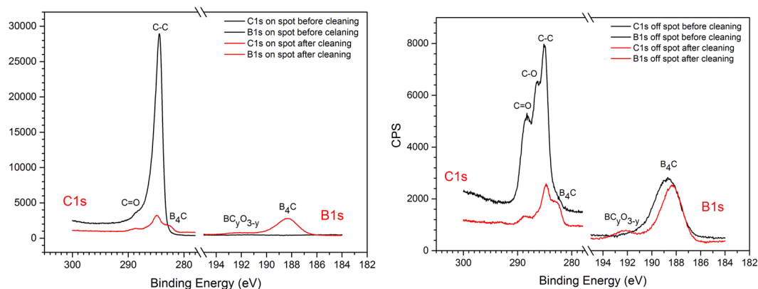
Figure 9. High-resolution C1s and B1s XPS spectra of the B_4C -coated test wafer before (black solid lines) and after pure O_2 RF plasma cleaning (red solid lines). Left panel: XPS data taken on the amorphous carbon contamination spot. Right panel: XPS data taken off the amorphous carbon contamination spot on the bare B_4C coating.
