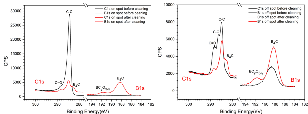
Figure 5. High-resolution C1s and B1s XPS spectra of the B_4C -coated test wafer before (black solid lines) and after H_2/Ar RF plasma cleaning (red solid lines). Left panel: XPS data taken on the amorphous carbon contamination spot. Right panel: XPS data taken off the amorphous carbon contamination spot on the bare B_4C coating.
