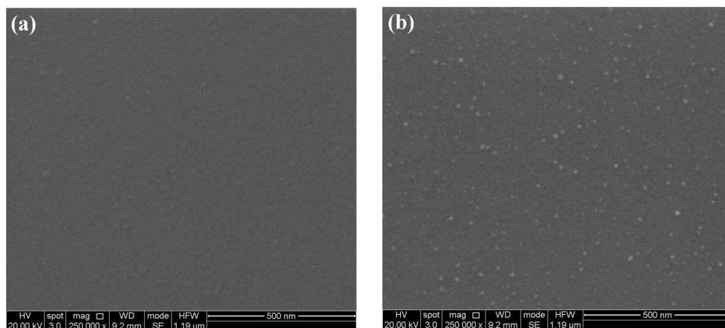
Figure 8. SEM images of B_4C -coated test wafers taken at 20 kV electron acceleration voltage with a 250 k-fold magnification after cleaning with H_2/Ar plasma: (a) Formerly a-C coated part, and (b) non a-C coated part.
