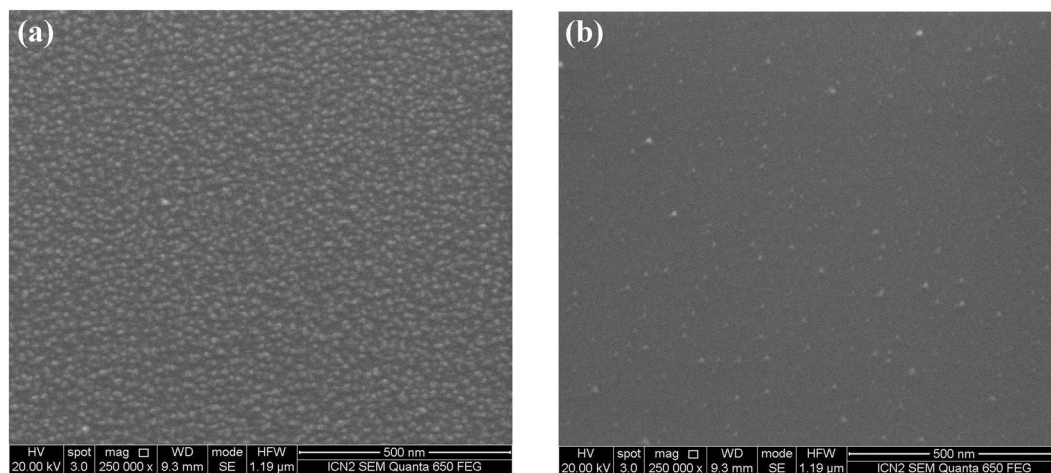
Figure 12. SEM images of B_4C -coated test wafers taken at 20 kV electron acceleration voltage with a 250k-fold magnification after cleaning with pure O_2 plasma: (a) Formerly a-C coated part, and (b) non a-C coated part.
