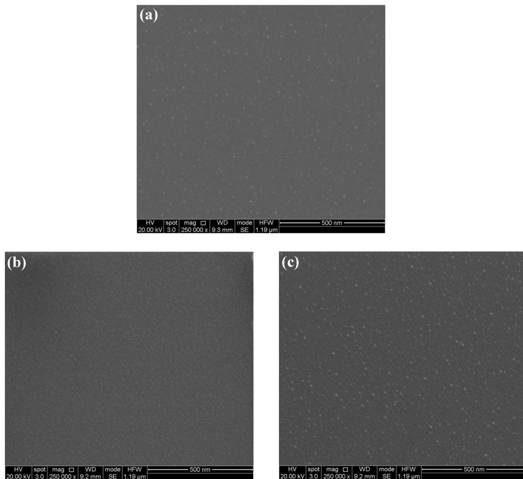
Figure 4. SEM images of B_4C -coated test wafers taken at 20 kV electron acceleration voltage with a 250 k-fold magnification: (a) Pristine B_4C -coated test wafer, (b) O_2/Ar -plasma cleaned – formerly a-C coated part, and (c) O_2/Ar -plasma cleaned – non a-C coated part.
