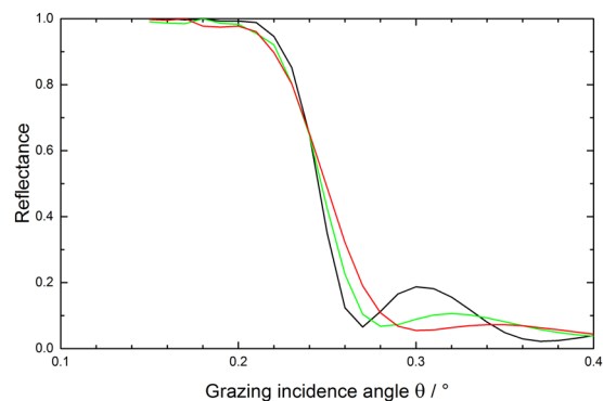
Figure 7. Comparison of XRR total reflection data at low grazing incidence angles for a pristine B_4C -coated test mirror (black line) and after a-C coating plus subsequent H_2/Ar plasma cleaning (green line: formerly a-C coated area; red line: non a-C coated area).
