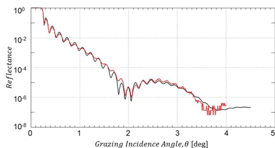
Figure 10. XRR data from B_4C -coated test mirror after cleaning with pure O_2 plasma cleaning. (red solid lines: experimental XRR data; black solid lines: IMD simulation).
