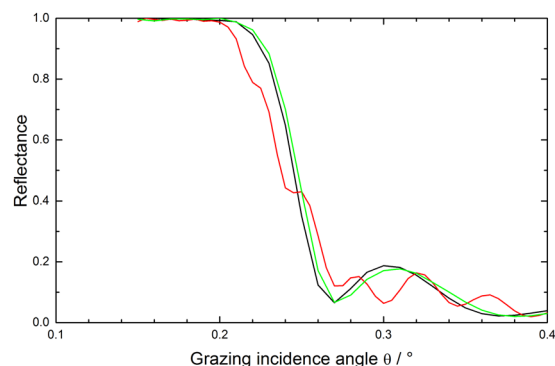
Figure 11. Comparison of XRR total reflection data at low grazing incidence angles for a pristine B 4 C-coated test mirror (black line), after a-C coating (red line), and after subsequent cleaning with pure O 2 plasma (green line).
