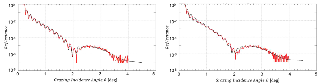
Figure 2. XRR data from B_4C -coated test mirror right after O_2/Ar plasma cleaning. Left hand side: Non a-C coated part; right hand side: Formerly a-C coated part (red solid lines: experimental XRR data; black solid lines: IMD simulation).
