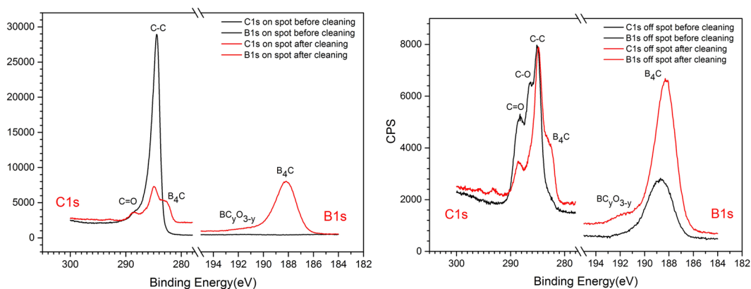
Figure 1. High-resolution C1s and B1s XPS spectra of the B 4 C-coated test wafer before (black solid lines) and after O 2 /Ar RF plasma cleaning (red solid lines). Left panel: XPS data taken on the amorphous carbon contamination spot. Right panel: XPS data taken off the amorphous carbon contamination spot on the bare B 4 C coating.
