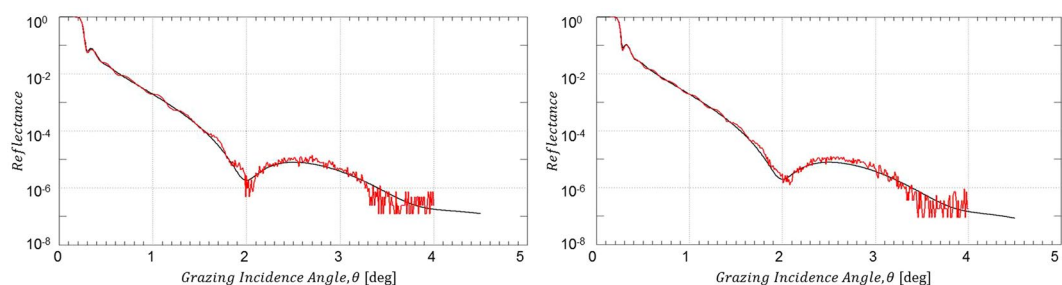
Figure 6. XRR data from B_4C -coated test mirror right after H_2/Ar plasma cleaning. Left hand side: Non a-C coated part; right hand side: Formerly a-C coated part (red solid lines: experimental XRR data; black solid lines: IMD simulation).
