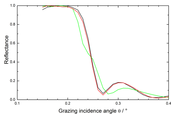
Figure 3. Comparison of XRR total reflection data at low grazing incidence angles for a pristine B 4 C-coated test mirror (black line) and after a-C coating plus subsequent O 2 /Ar plasma cleaning (green line: formerly a-C coated area; red line: non a-C coated area).
