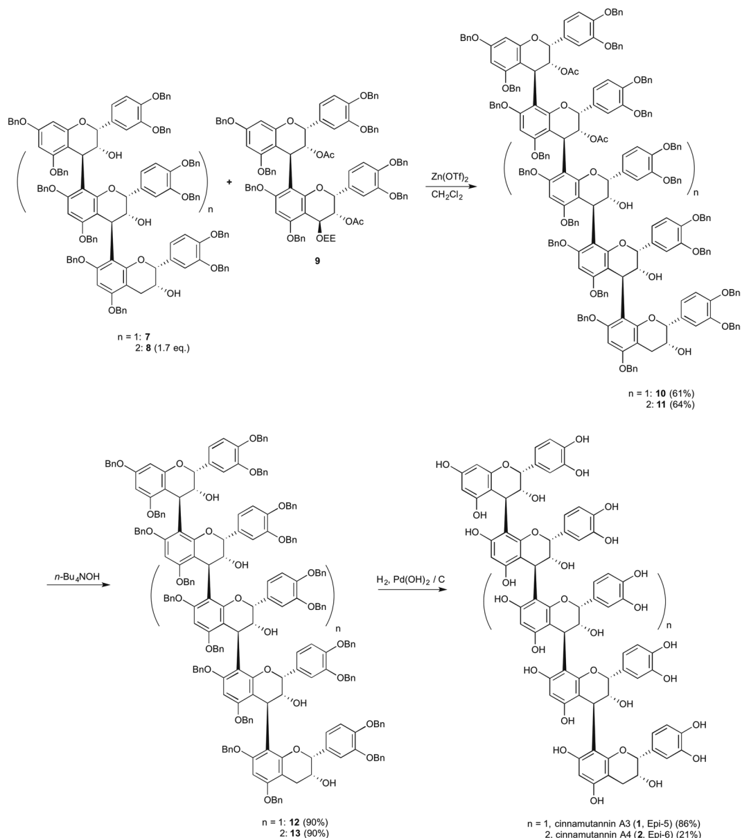
Figure 2. Synthesis of cinnamtannin A3 (1, Epi-5) and A4 (2, Epi-6). Cinnamtannin A3 (1, Epi-5) and A4 (2, Epi-6) were synthesized using \text{Zn}(\text{OTf})_2 mediated condensation. Ac, acetyl, Bn, benzyl, Bu, butyl, EE, ethoxyethyl, \text{Zn}(\text{OTf})_2 , HPLC, high performance liquid chromatography, zinc(II) trifluoromethanesulfonate, Bn, benzyl.
