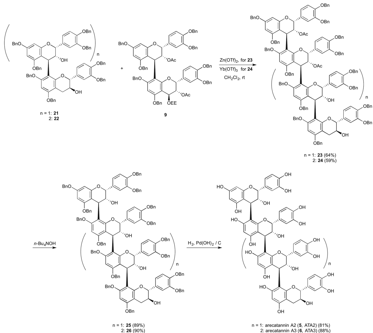
Figure 4. Synthesis of arecatannin A2 ( 5 , ATA2) and A3 ( 6 , ATA3). Arecatannin A2 ( 5 , ATA2) and A3 ( 6 , ATA3) were synthesized using \text{Zn}(\text{OTf})_2 and \text{Yb}(\text{OTf})_3 mediated equimolar condensation. \text{Yb}(\text{OTf})_3 , ytterbium trifluoromethanesulfonate.
