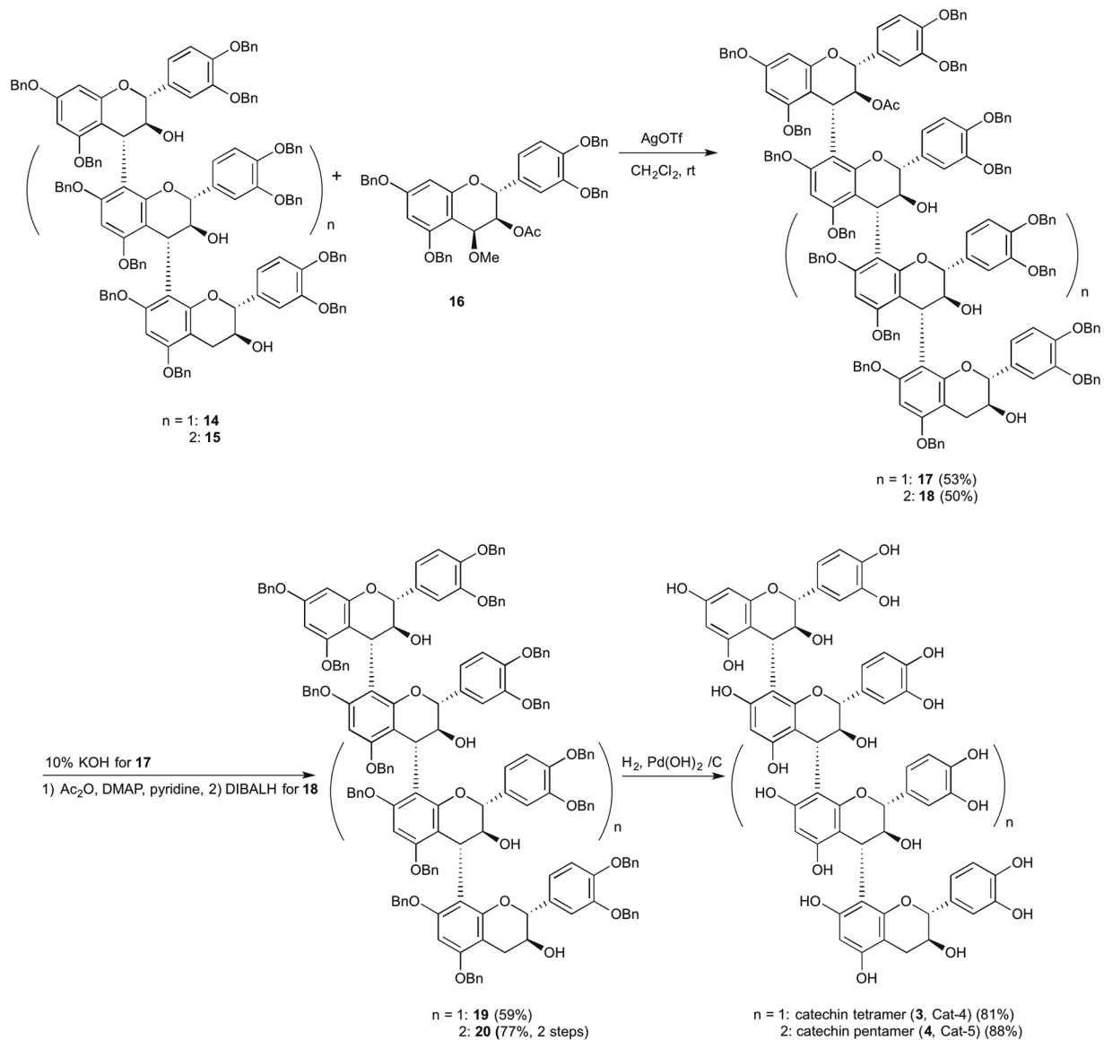
Figure 3. Synthesis of catechin tetramer ( 3 , Cat-4) and pentamer ( 4 , Cat-5). Catechin tetramer ( 3 , Cat-4) and pentamer ( 4 , Cat-5) were synthesized using AgOTf mediated equimolar condensation. AgOTf, silver trifluoromethanesulfonate, DIBALH, diisobutylaluminium hydride, DMAP, N, N, dimethyl-4-aminopyridine.
