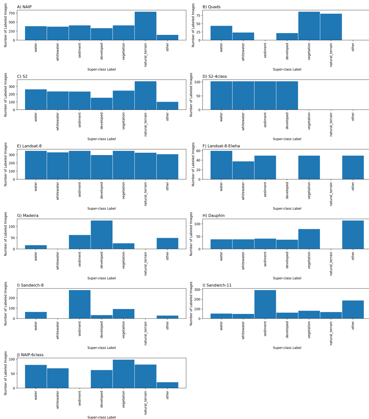
Fig. 7 Frequency distribution of images labeled by superclass label. We define a superclass as a broad class name for a collection of component classes. There are seven superclass labels, and between four and 12 class labels depending on the dataset. Hence the empty bars in some of the frequency histograms shown. Computer codes are provided that generate superclass label image sets.
