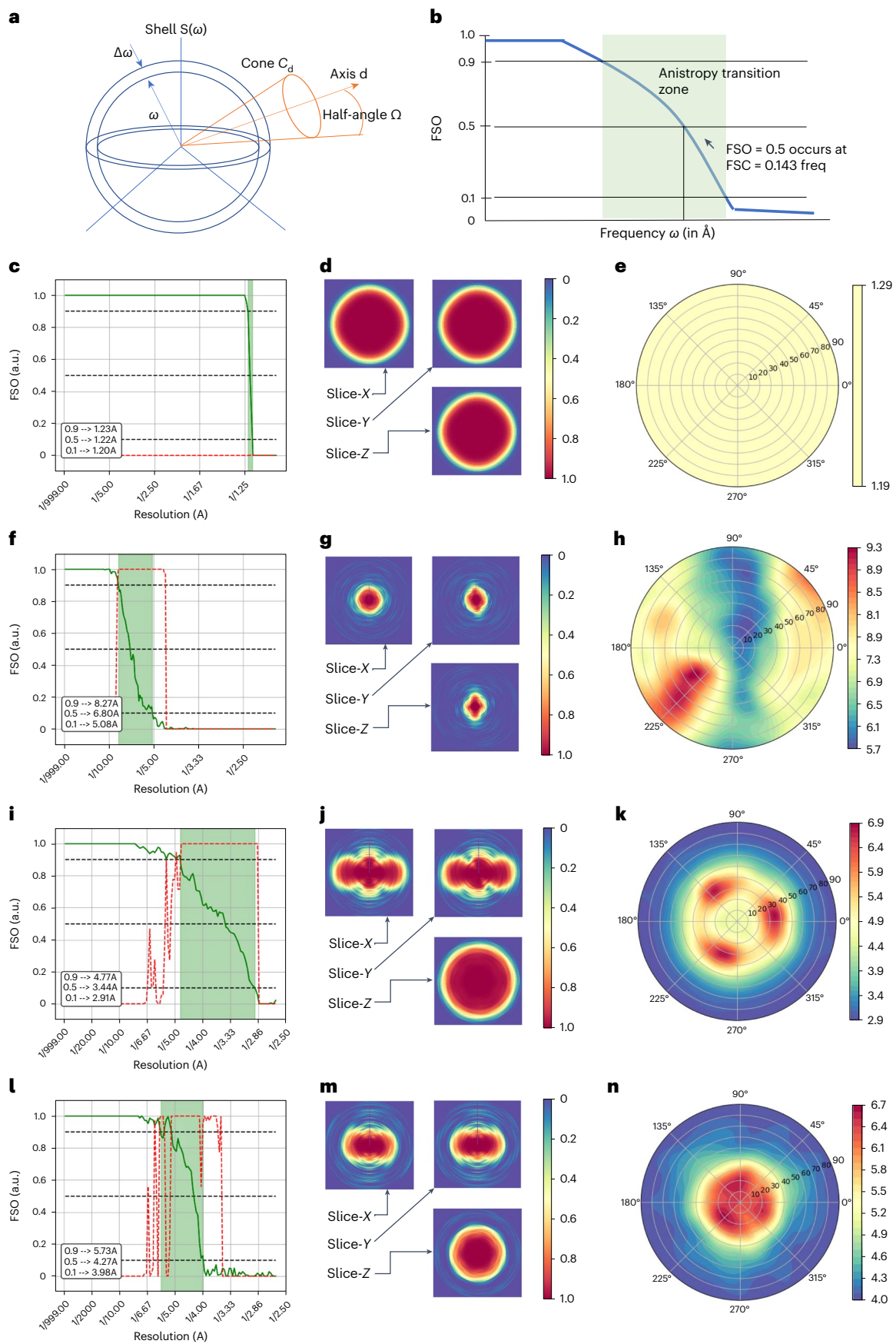
Fig. 1 | Anisotropy analysis. a , Scheme of directional FSC measurement. b , Description of the FSO curve. c–e , Apoferritin. f–h , Human CMG bound to AND-1. i–k , Influenza hemagglutinin trimer untilted map. l–n , Influenza hemagglutinin trimer tilted map. c, f, i, l , FSO (in continuous) and P value for the
