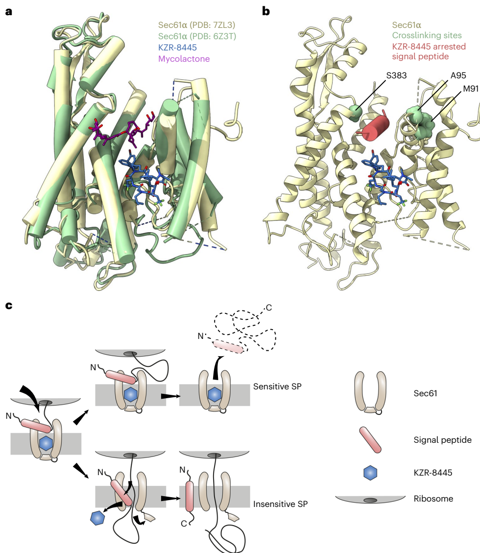
Fig. 5 | Proposed model for substrate-selective Sec61 inhibition.
