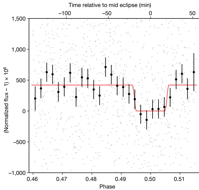
Fig. 1 | Eclipse light curve of TRAPPIST-1 c taken with MIRI F1500W. The phase-folded secondary eclipse light curve of TRAPPIST-1 c, measured with the MIRI imager at 15 \mu\text{m} . The eclipse is centred at orbital phase 0.5 and has a measured depth of f_p/f_s = 421 \pm 94 ppm. The light curve includes four visits (that is, four eclipses), each spanning approximately 3.2 h. To make the eclipse more easily visible, we binned the individual integrations (grey points) into 28 orbital phase bins (black points with 1\sigma error bars). The light curve was normalized and divided by the best-fit instrument systematic model. The best-fit eclipse model is shown with the solid red line. The data and fit presented in this figure are based on the SZ reduction, one of the four independent reductions we performed in this work.
