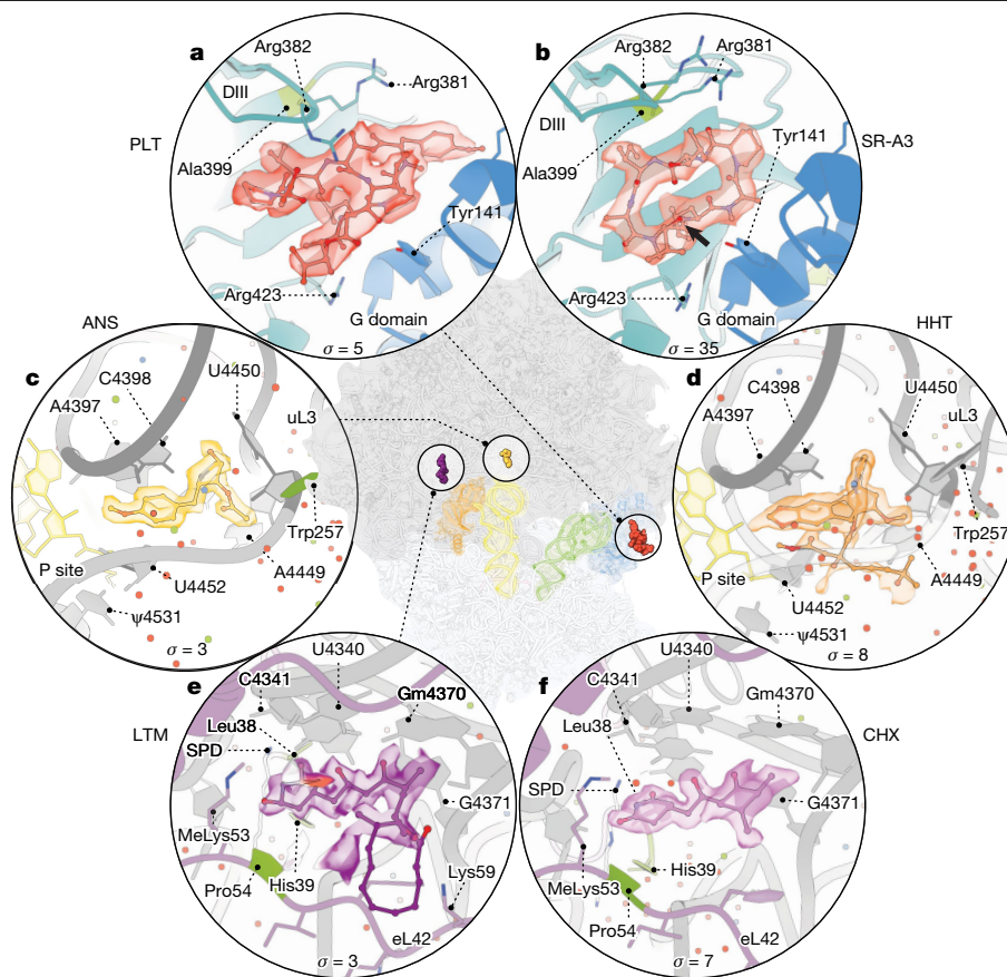
Fig. 5 | Binding sites for ribosome inhibitors. a, b , Overview of the binding sites for PLT (red) ( a ) and SR-A3 (coral) ( b ) on eEF1A between domain III (DIII, cyan) and the G domain (blue) bound to a GA-ribosome complex. Focus refined on eEF1A. The black arrow indicates the hydroxyl moiety that differentiates SR-A3 from ternatin-4. c–e , Structures of ANS (light orange) ( c ) and HHT (orange) ( d ) in the PTC and LTM (dark purple) ( e ) and cycloheximide (CHX, purple) ( f ) in
