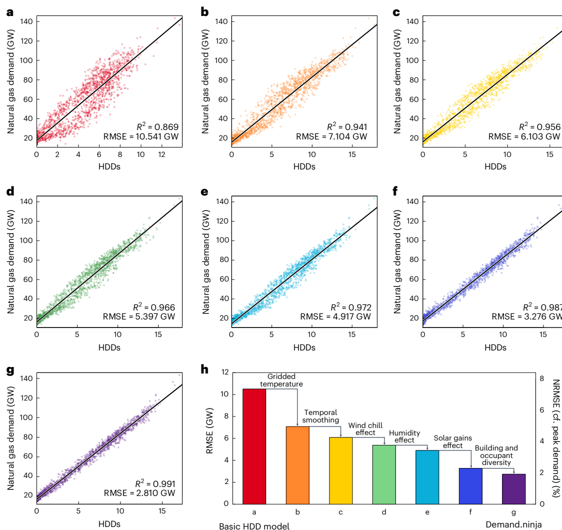
Fig. 3 | Ability of the Demand.ninja to model UK natural gas demand at daily resolution. a–g , The correlation between modelled HDDs and measured gas demand covering all end uses excluding power generation from ref. 78 over the period 2015–2019. Points show demand on individual days and lines show the derived linear regressions ( n = 1,827 ). Each panel shows incrementally more sophisticated models, starting with the most common elements and moving to the most novel. a , A basic degree-day model using the national average temperature. b , Degree days calculated using gridded temperatures that have been population weighted. c , The addition of smoothing temperatures over the preceding two days. d , The addition of wind chill (higher wind speeds reducing the temperature index). e , The addition of humidity effect (greater humidity
