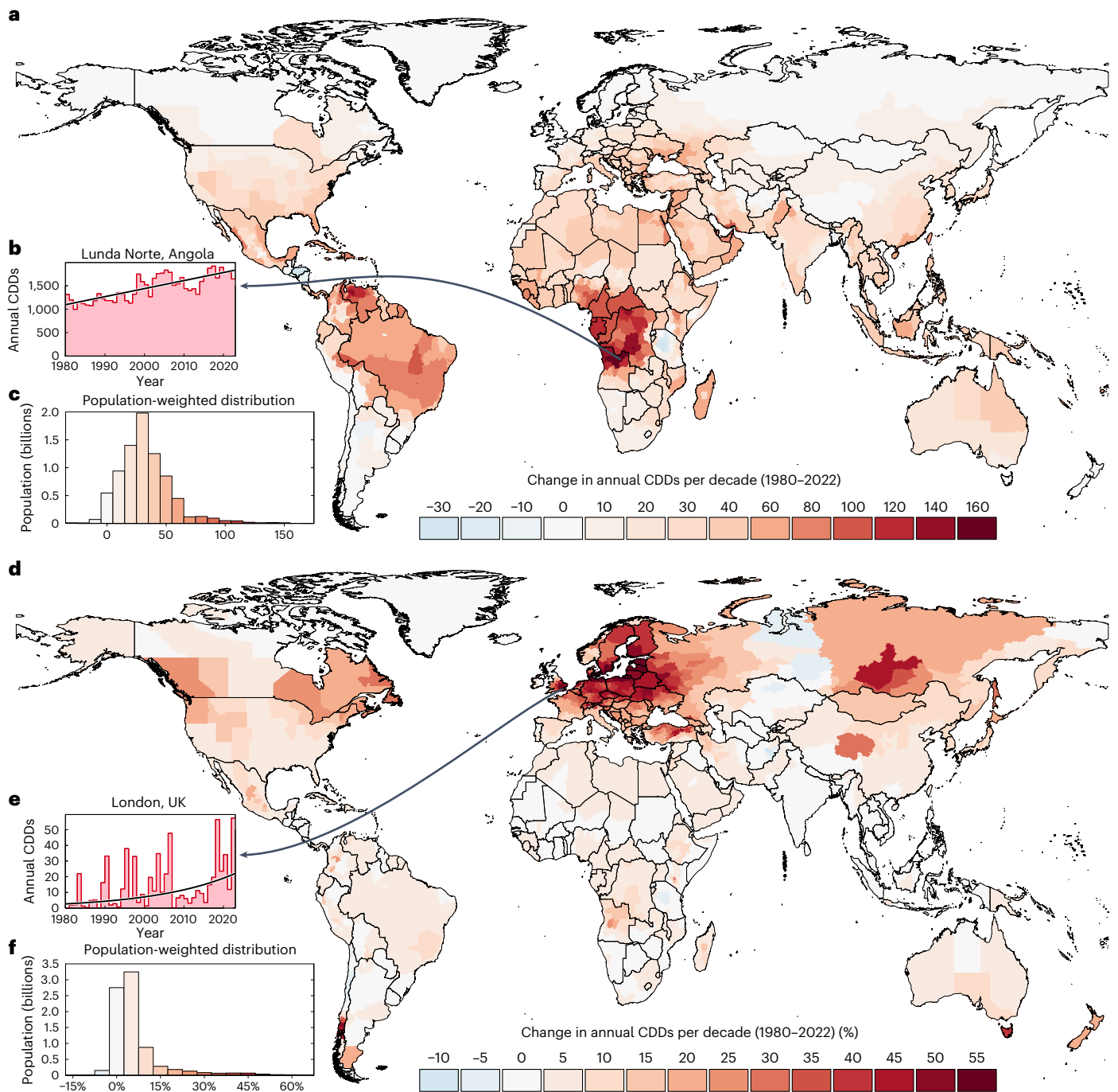
Fig. 8 | Global maps of the change in annual CDDs over the last four decades. All countries are modelled with a cooling threshold of 20 °C derived from our global calibration. a , The increase in absolute annual CDDs per decade, determined through linear regression of data from 1980 to 2022. d , The relative increase in CDDs per decade, determined through log-linear regression of data from 1980 to 2022. CDDs are evaluated at the level of administrative subregions (that is states, provinces) within larger countries (Methods). b, e , The 43 year time series of annual CDDs for two exemplary regions in Angola and the United Kingdom, which experience large absolute and relative increases respectively.
