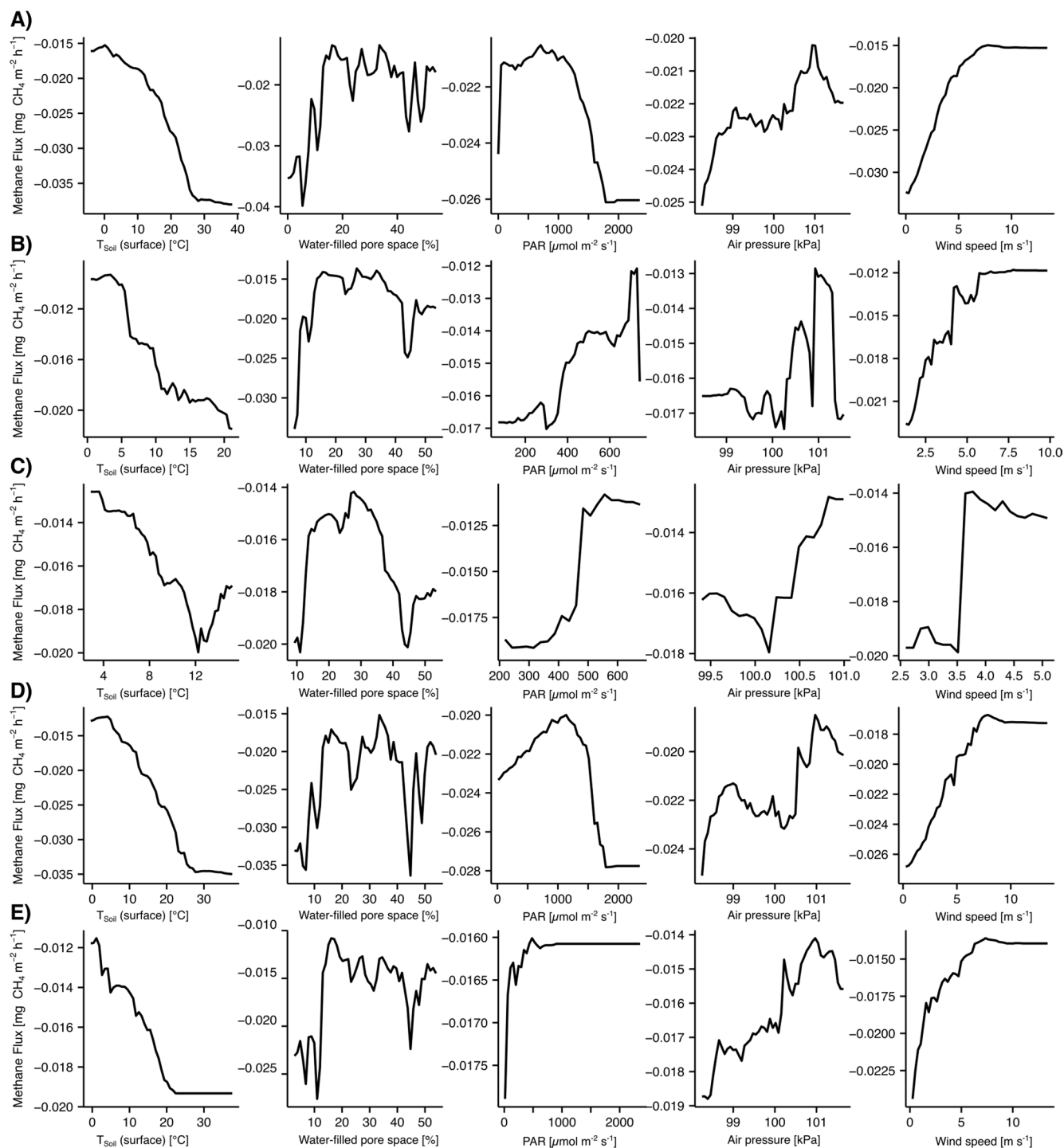
Extended Data Fig. 4 | Partial dependence plots of abiotic variables in Random Forest model. Partial dependence plots as outcome of the Random Forest (RF) models in Fig. 3a and Extended Data Fig. 3, for all vegetation types (18 chambers). Plots show the dependence of methane fluxes on surface soil temperature ( T_{\text{Soil}} (surface)), water-filled pore space, photosynthetically active
