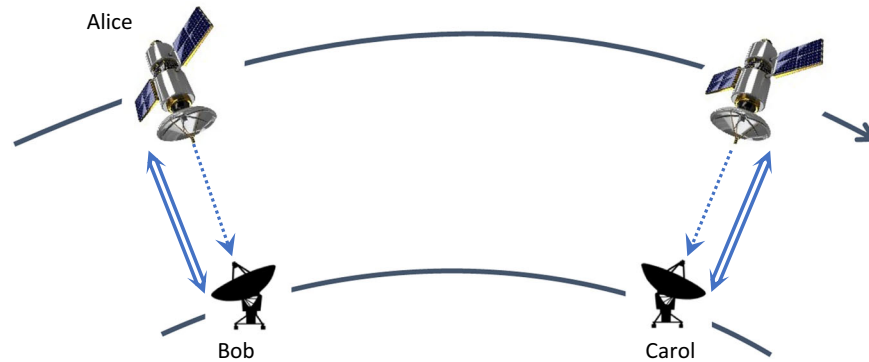
Fig. 1 Long-range quantum key exchange with satellite as trusted node. The dotted arrows represent quantum channels between the satellite (Alice) and each of the users (Bob and Carol). The white arrows represent classical public discussion channels, used to process the keys. By using both quantum channels and discussion channels, Bob and Carol can build a secret shared key. However, this secret key is also known to Alice, who therefore must be trusted by the parties.
