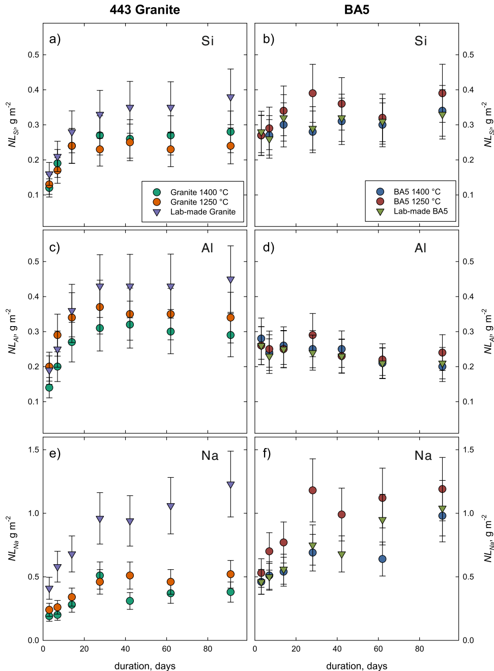
Fig. 3 The normalized mass loss ( NL_i ) for 443 Granite and BA5 samples from modified PCT-B conducted at 90^\circ\text{C} and 200\text{ m}^{-1} . NL_{\text{Si}} , NL_{\text{Al}} , and NL_{\text{Na}} are plotted in (a,c,e) and (b,d,f) for Granite 443 and BA5, respectively. The y-axis for the Na data (e,f) is plotted on a different scale than Si (a,b) and Al (c,d). The uncertainty displayed in the plots is 21% of the value of NL_i , was calculated with Eq. 6.
