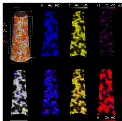
Fig. 8 Formation of nanoscale Pt surface segregates and elimination of core-shell distribution of AgAu. Concentration maps taken from 5 nm-thick slices of APT volumes of NPG-Pt air-annealed at 300 °C for 2 h, along the longitudinal axis. Scale bar is 30 nm.
