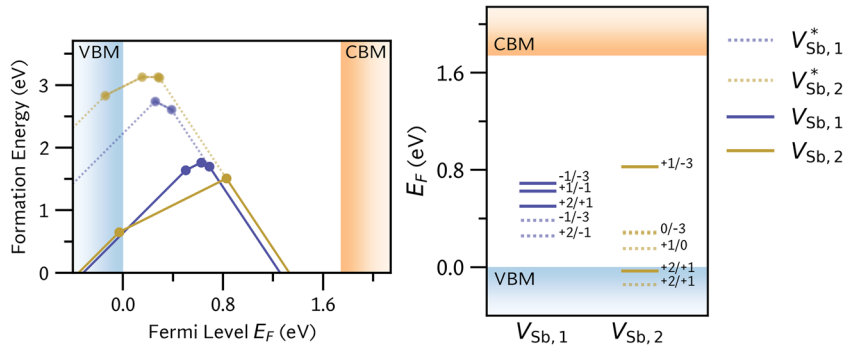
Fig. 6 Defect formation energy (left) and vertical energy level (right) diagram for the antimony vacancies in \text{Sb}_2\text{S}_3 , under sulfur rich conditions 121 ( \mu_{\text{S}} = 0 , \mu_{\text{Sb}} = -0.55 eV). The two symmetry inequivalent sites are depicted in purple ( V_{\text{Sb},1} ) and gold ( V_{\text{Sb},2} ). For each site, the ground state structures are shown with solid lines ( V_{\text{Sb}} ), while the metastable states are shown with faded dotted lines ( V_{\text{Sb}}^* ). The valence band maximum (VBM) and conduction band minimum (CBM) are shown in blue and orange, respectively.
