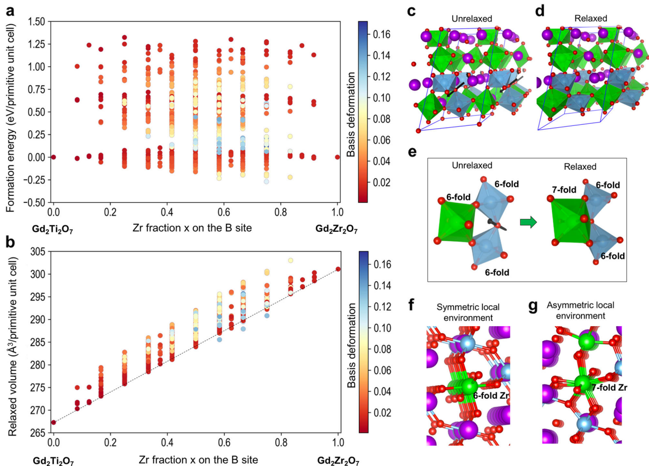
Fig. 3 a Basis deformation mapped DFT-computed mixing energies and b relaxed volumes (normalized to a primitive cell containing 22 atoms, i.e. , 2 effective pyrochlore formula units) as a function of composition. The colors represent the extent of the basis deformation. The dashed line in b represents a Vegard's law based interpolation. c, d Unrelaxed and DFT-relaxed supercell geometries for the \text{Gd}_2(\text{Zr}_{0.75}\text{Ti}_{0.25})_2\text{O}_7 ground-state structure. The relaxation of O atoms that are largely responsible for the large basis deformation are identified with black arrows (these structures are the same as shown in Fig. 1, just a different perspective and with fewer periodic images). e A closer view of the coordination environment changes as a result of the large O relaxations for the ground-state configuration. The coordination environment of the Zr atom changes from 6-fold to 7-fold, while the two Ti atoms remain 6-fold coordinated, although with slightly distorted octahedra. f, g Two representative cases from the DFT-computed dataset where local symmetry breaking around the Zr atoms drives the predicted large O relaxation behavior. When this symmetry breaking does not occur (as in f ), the O atoms do not relax so significantly
