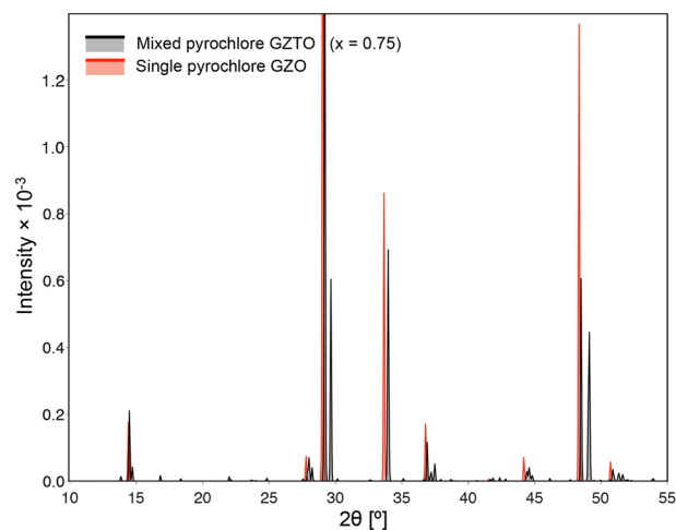
Fig. 2 Simulated XRD patterns for mixed GZTO, using the DFT-computed ground-state structure with x = 0.75 (black), and GZO (red) pyrochlores. CrystalDiffact was used to simulate the theoretical XRD patterns from the pyrochlore supercell geometries 43 and an orthogonalized supercell was used for simulating the XRD spectra 44
