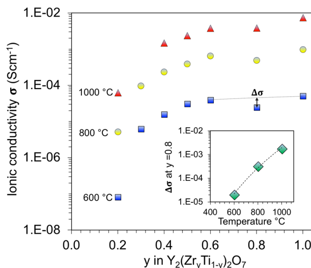
Fig. 7 Experimentally measured ionic conductivity \sigma for \text{Y}_2(\text{Ti}_{1-y}\text{Zr}_y)_2\text{O}_7 solid solutions as a function of temperature and Zr content y . Data is replotted from ref. 45 . Inset shows the temperature variation of \Delta\sigma , defined as the relative lowering of the ionic conductivity at y = 0.8 with respect to a value directly computed by a linear interpolation of the conductivity of the neighboring compositions
