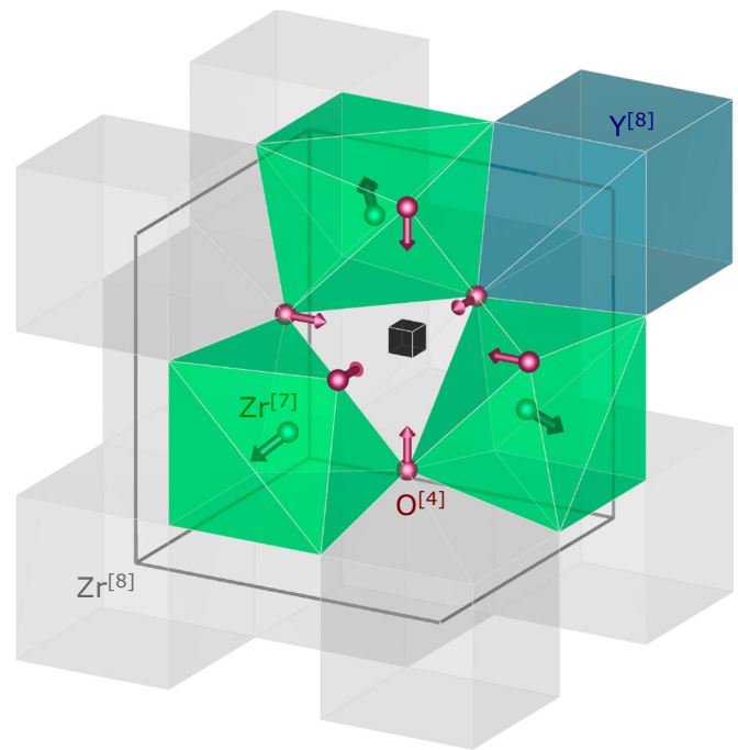
Fig. 1 | Schematic defect model for cubic stabilised zirconia. Grey polyhedra indicate \text{Zr}^{4+} ions in regular 8-fold coordination. The solid black cube indicates a vacancy site. \text{Zr}^{4+} ions in 7-fold coordination are displaced away from the vacancy along the \langle 111 \rangle directions, indicated in green. \text{O}^{2-} ions directly next to the vacancy are displaced towards the vacancy along the \langle 100 \rangle directions, indicated in purple. A possible \text{Y}^{3+} site that is the next-nearest neighbour to the vacancy is indicated by the blue coordination polyhedron. Figure generated using Vesta 62 .
