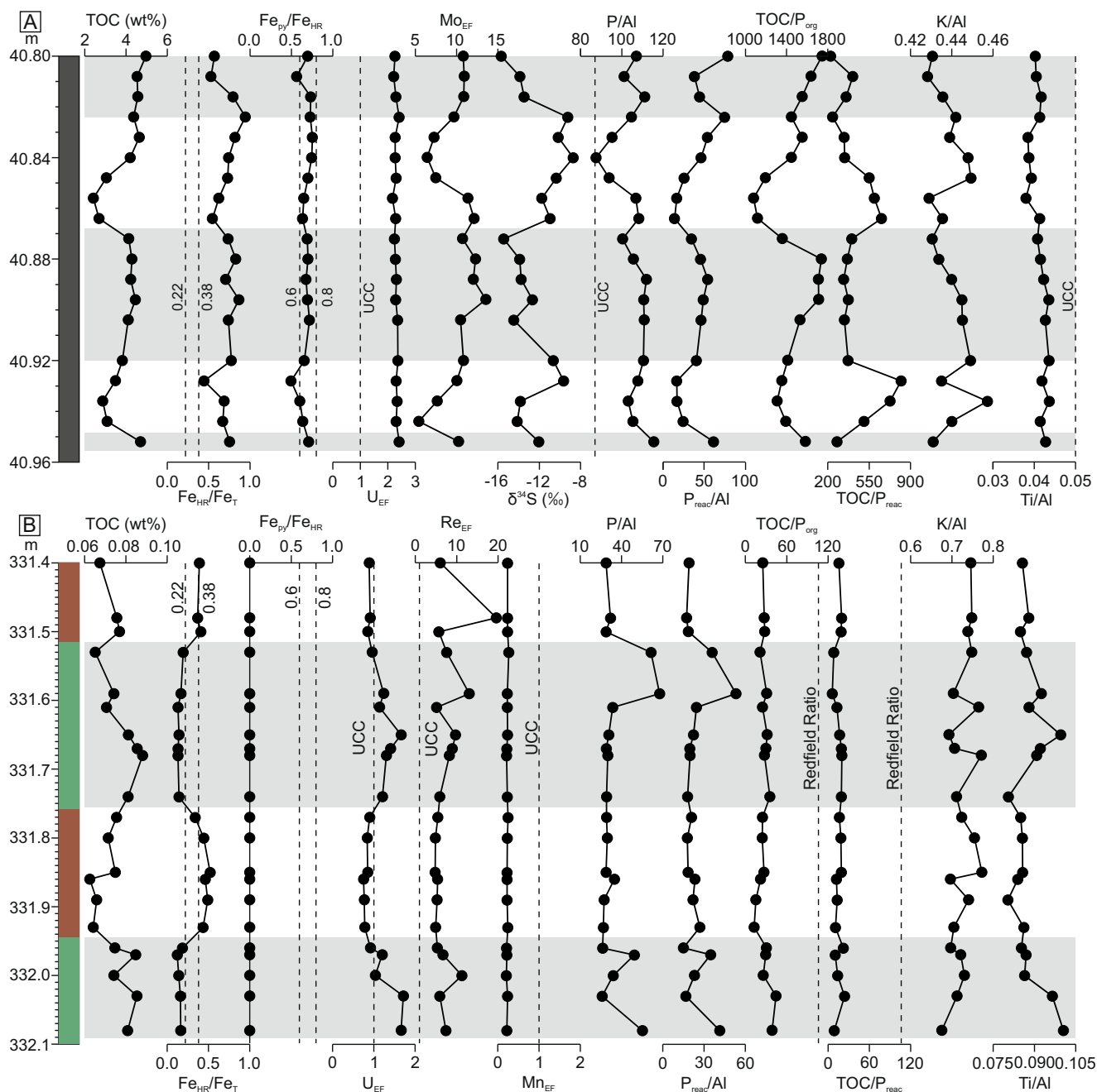
Fig. 2 | Geochemical and isotopic profiles. Section A, where shading indicates approximate position of cycles between lower total organic carbon (TOC) with more weakly sulfidic conditions (white), and higher TOC with more highly sulfidic conditions (gray). Section B, where shading corresponds to lithologic changes between red and green mudstones. Dashed lines on Fe_{HR}/Fe_T profiles represent calibrated thresholds indicative of oxic (<0.22) and anoxic (>0.38) water column conditions 3 , while dashed lines on Fe_p/Fe_{HR} profiles represent the lower (0.6) and
