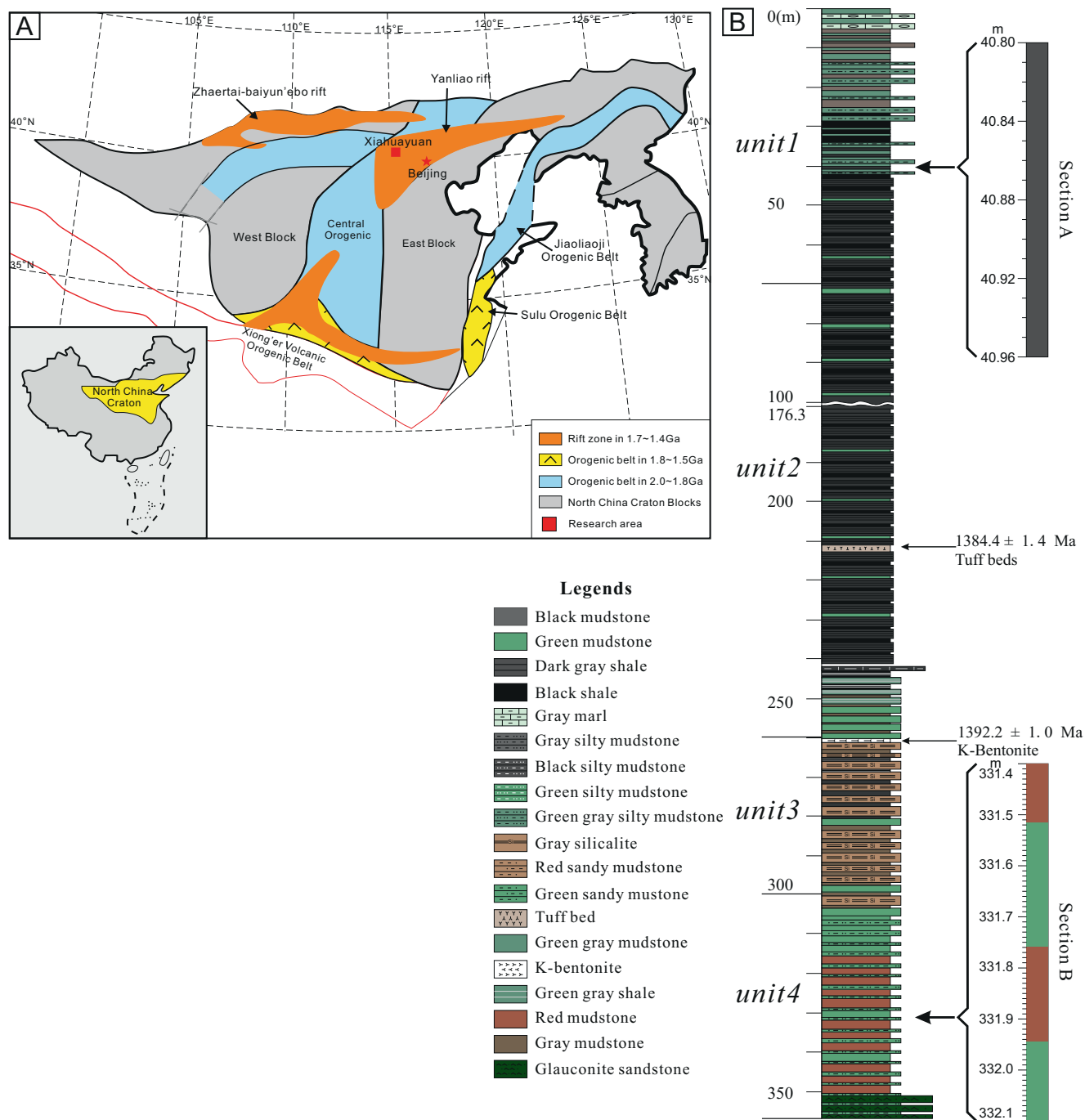
Fig. 1 | Simplified geological map and stratigraphy of the Xiamaling Formation. A Geological map of the North China Craton (NCC). Red square shows the study region. B Generalized stratigraphy of the 4 units of the Xiamaling Formation,
