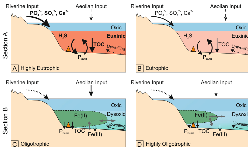
Fig. 3 | Schematic diagram highlighting fluctuating C-S-Fe-P systematics during deposition of eutrophic Section A and oligotrophic Section B. A Highly euxinic intervals in Section A experienced more intense runoff and organic matter burial. B Weakly euxinic intervals in Section A were driven by a relatively decreased riverine influx of sulfate and phosphate. C Deposition of Section B occurred within a ferruginous oxygen minimum zone (OMZ), with relatively increased aeolian inputs and upwelling under arid conditions promoting an expansion of the OMZ.
