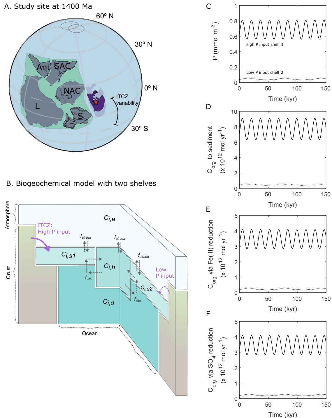
Fig. 4 | Conceptual framework and outputs of the multi-box biogeochemical model. A Paleogeographic reconstruction at -1.4 Ga, with red star indicating studied area. ITCZ: intertropical convergence zone. The ITCZ generally falls within -15° of the equator in both hemispheres 59,60 . L, Laurentia; Ant, Antarctica; SAC, South Australian Craton; NAC, North Australian Craton; S, Siberia. Purple polygon represents the NCC, with transparent outlines representing the approximate uncertainty from the (temporally) surrounding palaeomagnetic data. Green polygon approximates interconnected landmasses during the tenure of the supercontinent Nuna 51–63 . Longitude is unconstrained, and the two circles on the north pole represent palaeomagnetic data from Laurentia that constrain Nuna to a low-latitude position at this time 64 . B Conceptual framework for the multi-box biogeochemical model with two shelves (Shelf 1 is shown on the left, with a solid arrow indicating a higher input of P, while Shelf 2 is located on the right, with the dashed arrow indicating a lower input of P). Biogeochemical cycling in different boxes
