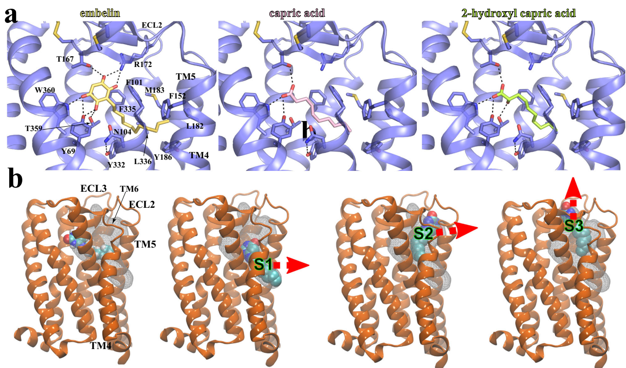
Fig. 5 | Docking of GPR84 agonists and MD simulations of 6-OAU-bound GPR84. a Interactions of docked embelin (light yellow), capric acid (pink), and 2-hydroxyl capric acid (lime) with GPR84 (slate). Hydrogen bonds are shown as black dashed lines. b Putative exit routes of 6-OAU in MD simulations. The 6-OAU movement
