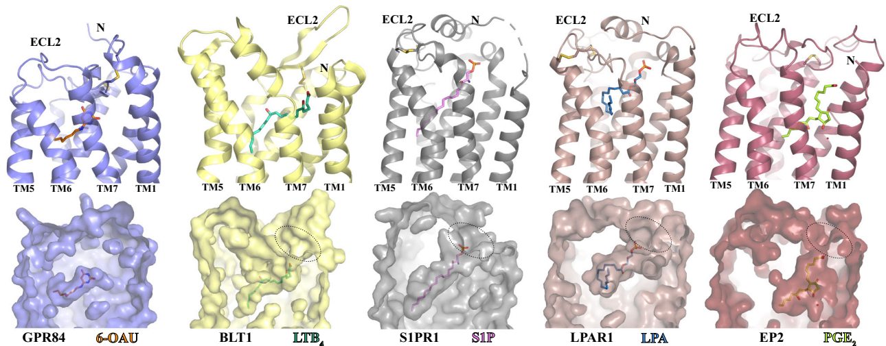
Fig. 4 | Comparison of the ligand-binding pockets in GPR84 and four other lipid GPCRs. BLT1, SIPRI, LPAR1, and EP2 are receptors of \text{LTB}_4 , SIP, LPA, and \text{PGE}_2 , respectively. The structures of GPR84, BLT1 (PDB ID 7VKT), SIPRI (PDB ID 7TD3), LPAR1 (PDB ID 7TDO), and EP2 (PDB ID 7CX2) are colored slate, light yellow, gray,
