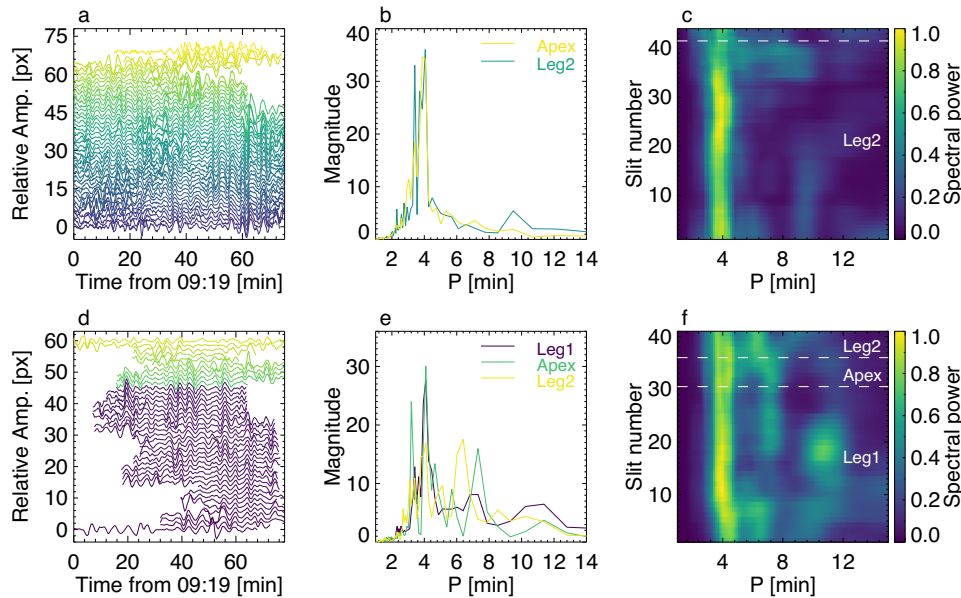
Fig. 3 | Analysis of observed kink oscillations. Oscillatory transverse displacements of different segments along the analysed loop (panels a and d , for HRIEUV and AIA, respectively), and their Fourier power spectra (panels b , c , e and f ). Panels a and d show the detrended oscillations signals, obtained by subtracting the trend from original displacements determined by the time–distance maps. The trend is obtained by smoothing the original signals with a window longer than the
