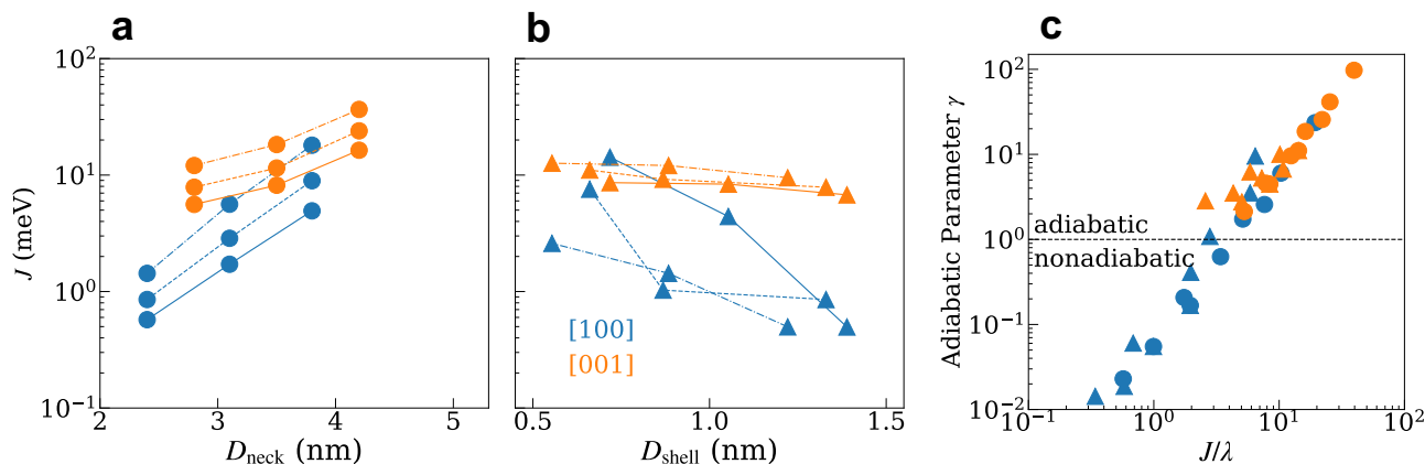
Fig. 2 | Electronic properties of the QD dimers. a, b Hybridization energy J of the ground donor and acceptor states as a function of neck width D_{\text{neck}} (a) and shell thickness D_{\text{shell}} (b) for [100] and [001] orientation attachments. Circle and triangle represent controlling the QD dimer by D_{\text{neck}} and D_{\text{shell}} , respectively. Solid, dashed, and dotted-dashed lines correspond to core diameters D_{\text{core}} of 2.2 nm, 3.0 nm, and
