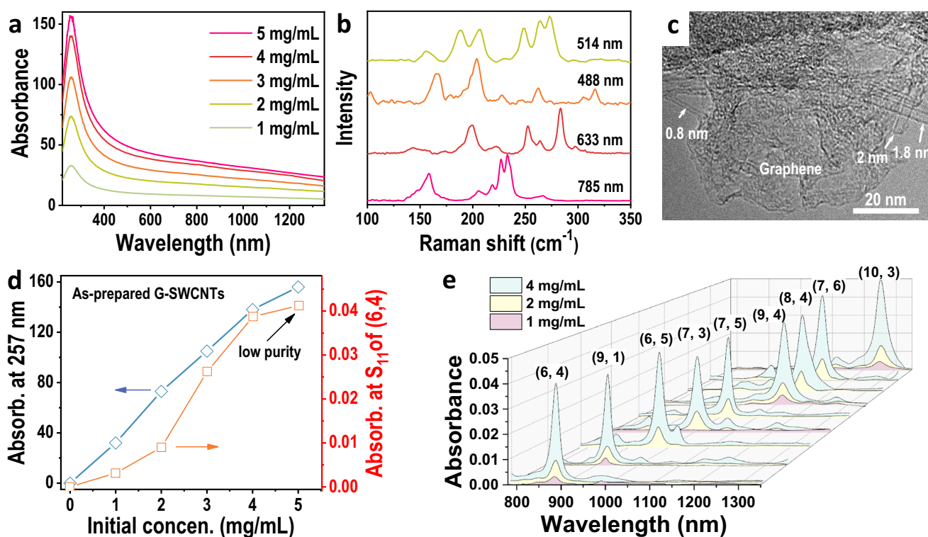
Fig. 3 | Dispersion and structure separation of high-concentration G-SWCNTs. a Optical absorption spectra of as-prepared G-SWCNTs with different concentrations. b Raman spectra of raw G-SWCNTs at excitation wavelengths of 514 nm, 488 nm, 633 nm, and 785 nm. c TEM image of raw G-SWCNTs containing graphene sheets and SWCNTs with different diameters. d Plot of the SWCNT concentration in the as-prepared dispersion (blue) and the corresponding yields of (6, 4) SWCNTs (orange) as a function of the initial concentration of G-SWCNTs. The resulting
