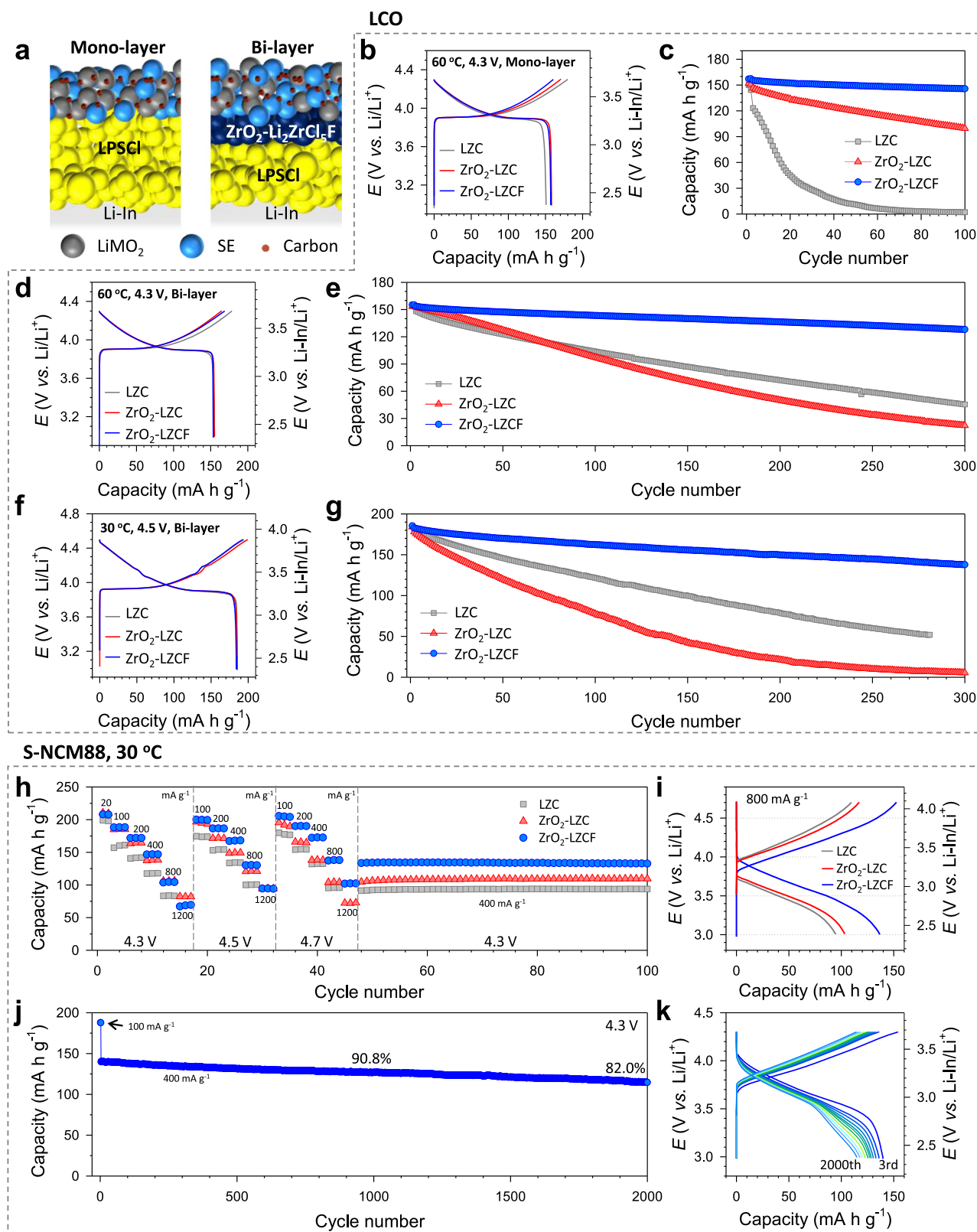
Fig. 5 | LCO and S-NCM88 ASSB cells employing HNSEs ( \text{ZrO}_2\text{-Li}_2\text{ZrCl}_5\text{F} and \text{ZrO}_2\text{-Li}_2\text{ZrCl}_6 vs. \text{Li}_2\text{ZrCl}_6 ). a Schematics of ASSB cells employing an LPSCI monolayer or ( \text{ZrO}_2\text{-LZCF} )/LPSCI bilayer. b, c First-cycle charge–discharge voltage profiles at 16.4 mA g -1 and 60 °C ( b ) and cycling performances at 82.0 mA g -1 ( c ) for LCO electrodes with an LPSCI monolayer cycled up to 4.3 V (vs. Li/Li + ). d–g First-cycle charge–discharge voltage profiles at 16.4 mA g -1 and cycling performances at 82.0 mA g -1 for LCO electrodes with a \text{ZrO}_2\text{-LZCF} bilayer cycled up to 4.3 V at 60 °C ( d, e ) and 4.5 V (vs. Li/Li + ) at 30 °C ( f, g ). h, i Rate capabilities with varying cut-off voltages ( h ) and the corresponding charge–discharge voltage profiles at 800 mA g -1
