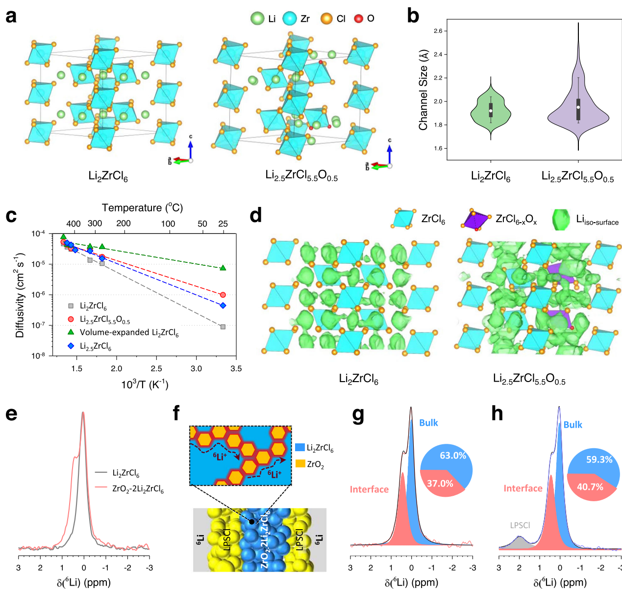
Fig. 3 | Interfacial Li + superionic conduction in HNSEs. a Crystal structures of \text{Li}_2\text{ZrCl}_6 and \text{Li}_{2.5}\text{ZrCl}_{5.5}\text{O}_{0.5} . b Topological analysis and channel size of \text{Li}_2\text{ZrCl}_6 and \text{Li}_{2.5}\text{ZrCl}_{5.5}\text{O}_{0.5} . The white circle, box and whisker indicate the mean value, values from the 25% to the 75% percentiles and values from the 10% to the 90% percentiles, respectively. c Arrhenius plots of the AIMD simulation extrapolated to 300 K. d Li
