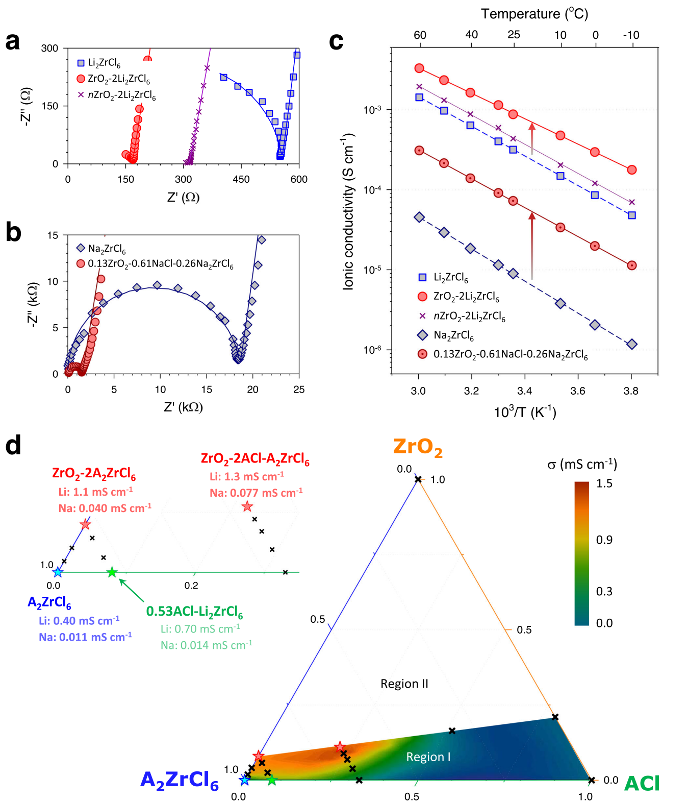
Fig. 2 | Ionic conductivities of \text{Li}^+ and \text{Na}^+ HNSEs ( \text{ZrO}_2\text{-}(\text{-ACl})\text{-A}_2\text{ZrCl}_6 ).
