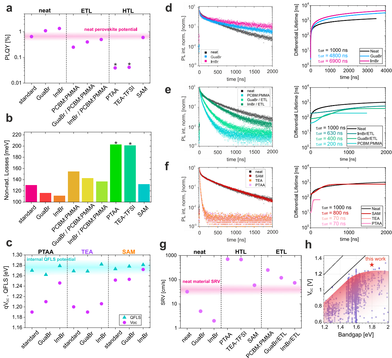
Fig. 4 | Charge recombination and energy losses. a PLQY results for different perovskite films and half-stacks (with either an ETL or HTL) illuminated with a 532 nm laser at a 1 sun equivalent intensity. The luminescence potential range of the neat perovskite on glass is highlighted in translucent pink. b Non-radiative recombination losses with respect to the radiative thermodynamic limit of the perovskite absorber calculated from the PLQY values reported in a . Details of the calculation can be found in SI . The asterisks in a , b indicate that the PLQY and non-radiative losses calculated for the PTAA and TEA-TFSI can be additionally affected by halide segregation, as discussed in Fig. S31. c QFLS- V_{oc} comparison on full devices extracted from PLQY maps presented in Figs. S37–39. Each QFLS value is calculated from a PLQY measurement on the same pixel from which the V_{oc} is
