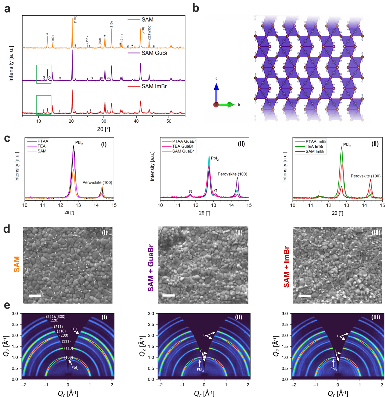
Fig. 3 | Structural and morphological characterization. a XRD patterns for neat SAM/perovskite films and after treatment with GuBr or ImBr. Additional experimental details in SI . Indices are for the cubic perovskite phase, and secondary phases are marked: \text{PbI}_2 with *, ITO with #, GuBr-induced phase with 'G' and ImBr-induced phase with 'I'. b Illustration of a mixed-halide 4H polytype, identified following the surface treatments (structure modified from reference Gratia et al. 33 ). c Highlighted regions comparing XRD for all (i) neat, (ii) GuBr-treated and (iii)
