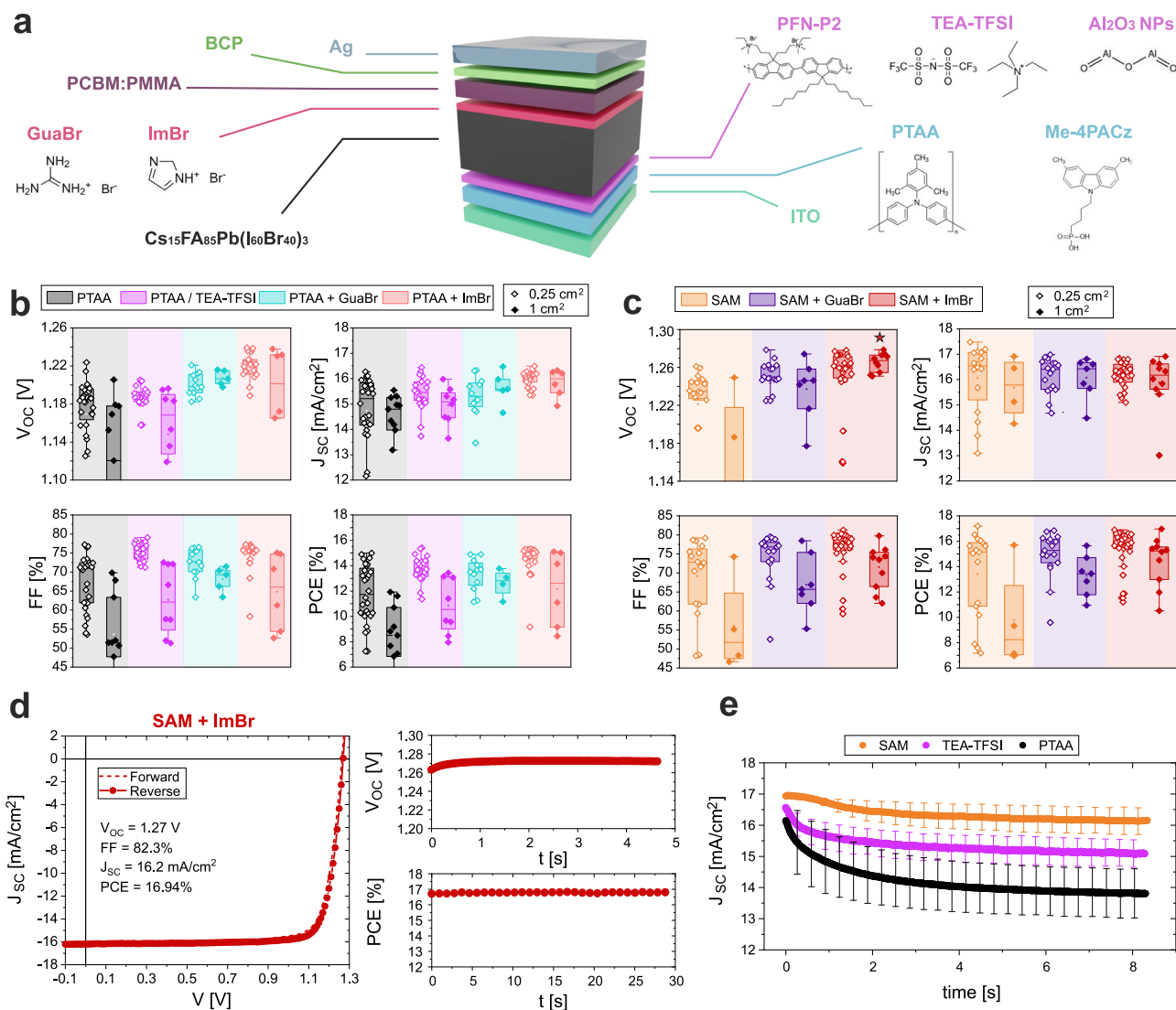
Fig. 2 | Device characterization. a Illustration of the typical 1.8 eV perovskite pin device used in this work. All the possible device architecture variations investigated in this study are also represented with their respective chemical structures. b Device statistic of a series of interface optimizations on perovskite devices using PTAA as the HTL obtained from reverse JV scans with a scan rate of 0.3 V/s. Here a PCE cut off was applied for devices with PCEs less than half of the mean value. c Performance metrics for surface-treated perovskite devices using Me-4PACz as the HTL, obtained from reverse JV scans with a scan rate of 0.3 V/s. Here a PCE cut off was applied for devices with PCE lower than half of the mean value. The star
