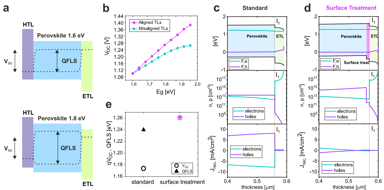
Fig. 1 | Drift-diffusion simulations. a Schematic diagram representing 1.6 eV and 1.8 eV perovskite solar cells using a hole and electron transport layer optimized for the 1.6 eV cell. The relation between the internal QFLS and external V_{OC} is indicated by the dotted lines. b V_{OC} obtained from drift-diffusion simulations for a perovskite solar cell device with varying energy gap. The purple data points represent a case where the energy levels of the transport layers are adjusted according to the perovskite bandgap in order to maintain ideal alignment, whereas the turquoise points illustrate the effect of the energy levels remaining the same as those optimized for
