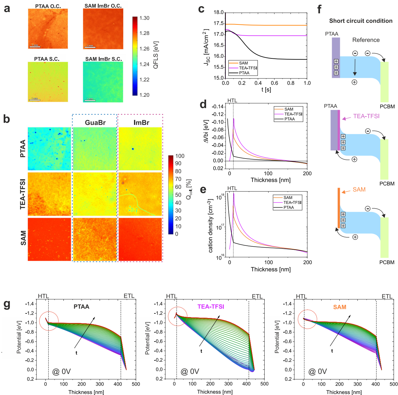
Fig. 5 | Charge collection and field screening. a QFLS mapping calculated from 3.7 \times 3.7 mm PLQY images for PTAA and SAM-ImBr devices recorded at V_{OC} and J_{SC} conditions. b Series of 3.7 \times 3.7 mm images obtained from PLQY images by illuminating a full device pixel under blue LED light at 1 sun equivalent. The images represent the quality of charge collection Q_{coll} by comparing the PLQY at V_{OC} and J_{SC} conditions. c Time-dependent drift-diffusion simulation results presenting the decay of J_{SC} over short timescales. d Variation of internal built-in voltage at 0 V from
