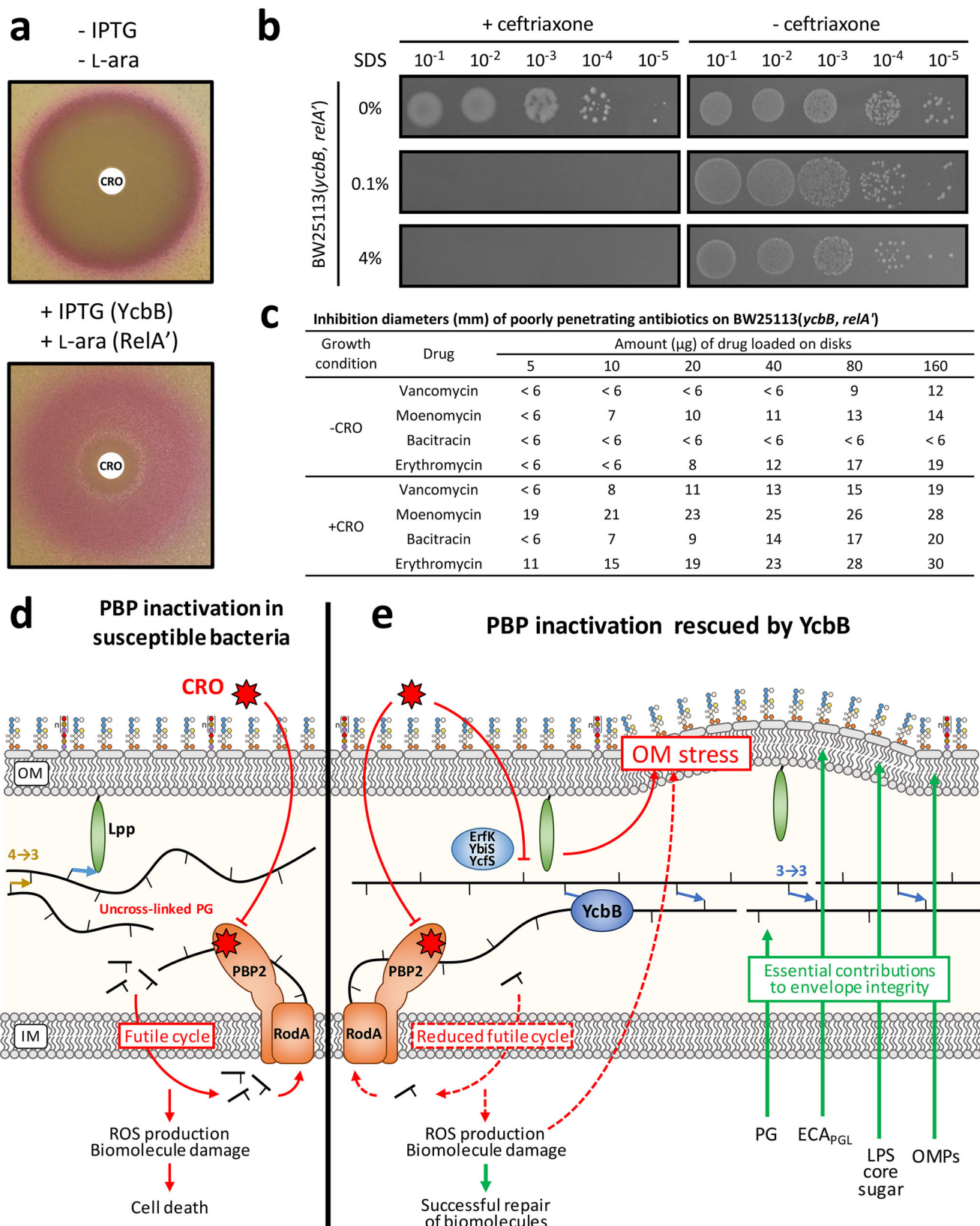
Fig. 6 | Testing outer membrane permeability in the presence of ceftriaxone. a Hydrolysis of chromogenic CPRG at 20 \mu\text{g}/\text{ml} by cytoplasmic LacZ 63 . The disks were loaded with 30 \mu\text{g} ceftriaxone. b Plating efficiency in the presence of SDS. Growth was tested in the presence of ceftriaxone at 8 \mu\text{g}/\text{ml} (+ceftriaxone) or in the absence of the drug (-ceftriaxone) on BHI agar plates supplemented with 40 \mu\text{M} IPTG and 1% L-arabinose for induction of ycbB and relA' , respectively. c Inhibition diameters of drugs that do not penetrate the outer membrane of wild-
