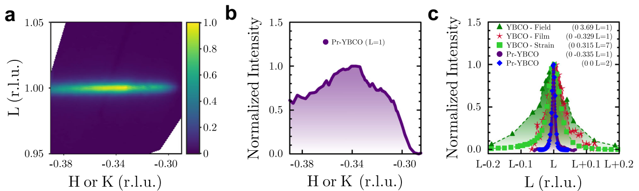
Fig. 2 | The reciprocal space structure of the 3D CO at T = 50 K. a An HL or KL reciprocal space map collected at 932.4 eV shows a diffraction feature centered at (0\text{-}0.335\ 1) reciprocal lattice units (r.l.u.). b A cut along H or K at L = 1 shows the peak is centered around a value of H or K = -0.335 (r.l.u.). c A comparison of the out-of-
