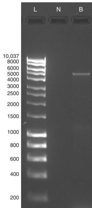
Fig. 4 PCR detection of the ICE_RbtetW_07 in Blautia schinkii DSM 10518. The expected amplicon size of the region from the virD4 gene to the tet(W) gene was 4794 pb. L: 1 kb HyperLadder, N: negative sample, and B: Blautia schinkii DSM 10518
