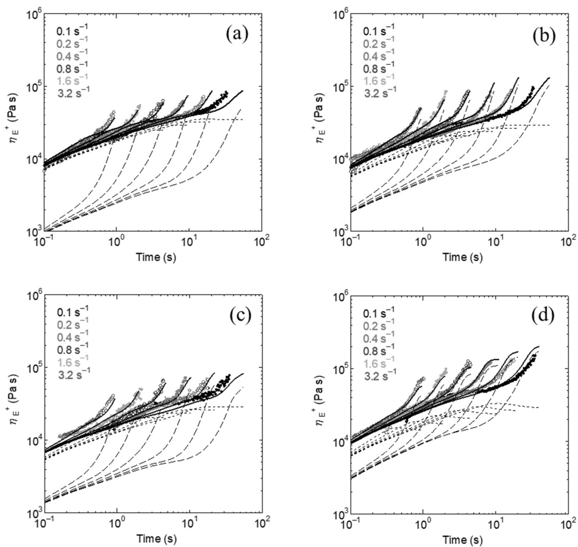
Fig. 4 Transient elongational viscosity \eta_E^+ with time at various Hencky strain rates at 190 °C for (a) PP/LDPE-M (85/15), (b) PP/LDPE-M (70/30), (c) PP/LDPE-L (70/30), and (d) PP/LDPE-H (70/30). The solid lines represent the numerical results. The contributions of the stress generated in PP (dotted lines) and LDPE (dashed lines) are also indicated
