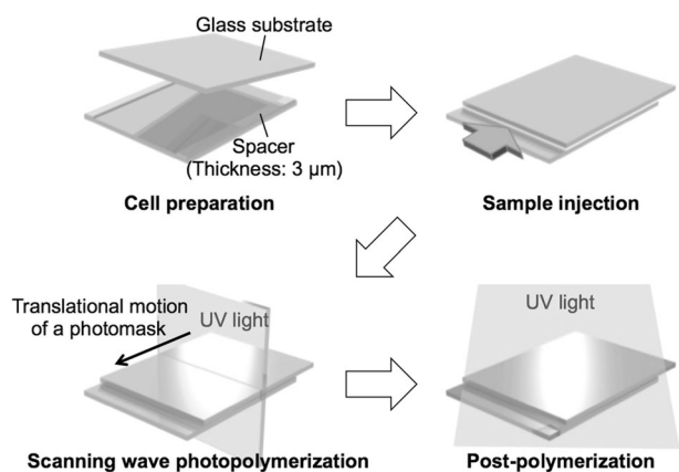
Fig. 2 Schematic illustrations of the procedure for fabricating an azobenzene-doped film
