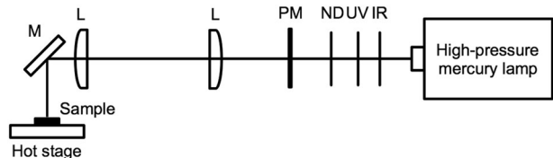
Fig. 3 Side view of the optical setup used for photopolymerization reactions. IR IR-cut filter, UV UV-bandpass filter, ND neutral-density filter, PM photomask, L plane convex lens, and M Mirror
