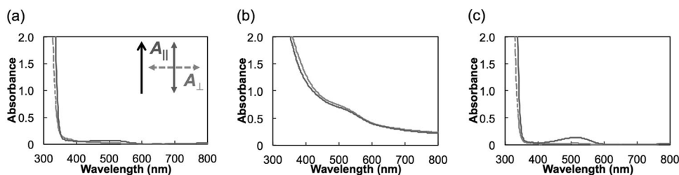
Fig. 6 Polarized UV-vis absorption spectra of the DR1-doped films obtained by photopolymerization at light intensities of 1.2 \text{ mW/cm}^2 (a), 0.2 \text{ mW/cm}^2 (b), and 1.2 \text{ mW/cm}^2 in the scanning wave
