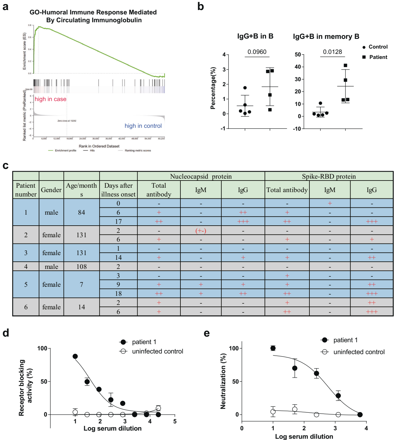
Fig. 1 Protective humoral immunity in SARS-CoV-2 infected pediatric patients. a Humoral immune response mediated by circulating immunoglobulin (GO:0002925); b Percentage of IgG+ B cells in CD19+ B cells and CD27+ memory B cells. The statistical method is the Student's t test. c Antibodies detection for nucleocapsid protein and receptor binding domain of Spike of SARS-CoV-2. +: positive, -: negative; (+-): weak negative. d Receptor-blocking activity of serum from an infected case and uninfected control. e Pseudovirus neutralizing assay of serum from an infected case and uninfected control. The statistical method is the Student's t test
