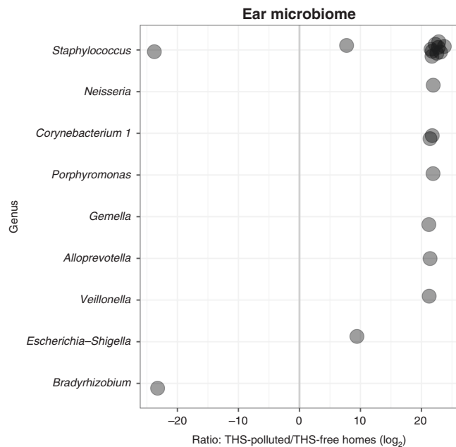
Fig. 3 Results of the log 2 -fold analysis based on the ASVs identified in the 16S sequencing libraries from ear samples. Each dot indicates a specific ASV taxonomically identified from the genus indicated on the Y-axis. Positive values on the X-axis indicate the ASV is significantly more abundant (FDR-adjusted p < 0.05 ) in THS-polluted homes (vTEG; n = 7 samples) than in THS-free (vNEG; n = 9 samples) homes, whereas negative values indicate the opposite. Only ASVs with log 2 -fold-change values > |5| are shown.
