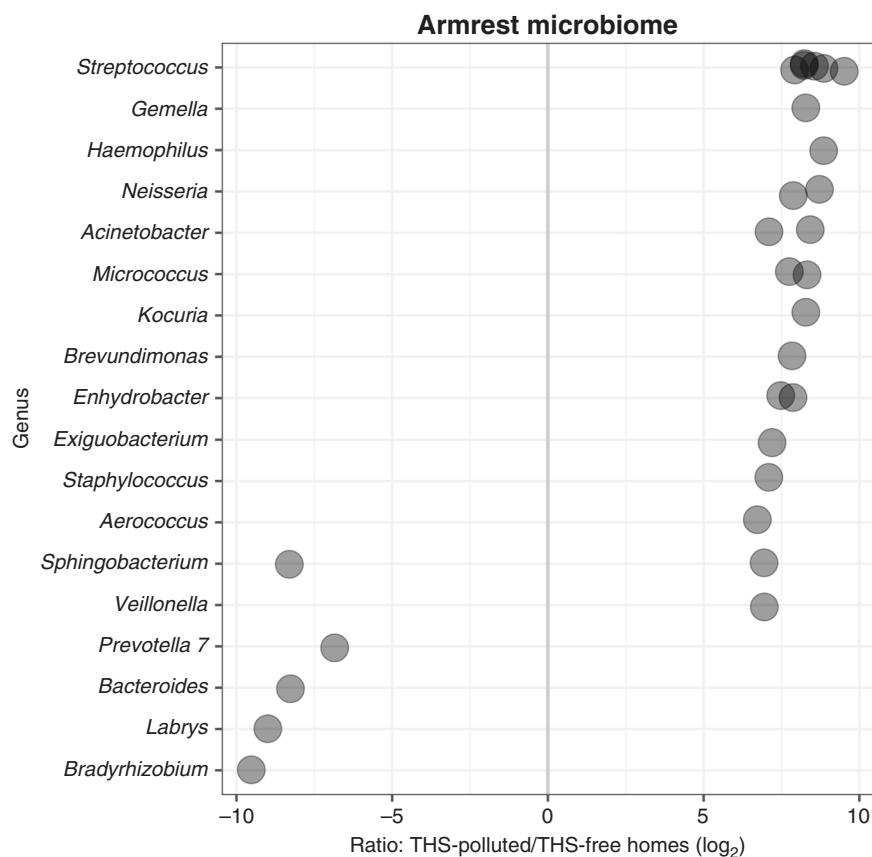
Fig. 4 Results of the log 2 -fold analysis based on the ASVs identified in the 16S sequencing libraries from armrest samples. Each dot indicates a specific ASV taxonomically identified from the genus indicated on the Y-axis. Positive values on the X-axis indicate the ASV is significantly more abundant (FDR-adjusted p < 0.05 ) in THS-polluted homes (vTEG; n = 4 samples) than in THS-free (vNEG; n = 8 samples) homes, whereas negative values indicate the opposite. Only ASVs with log 2 -fold-change values > |5| are shown.
