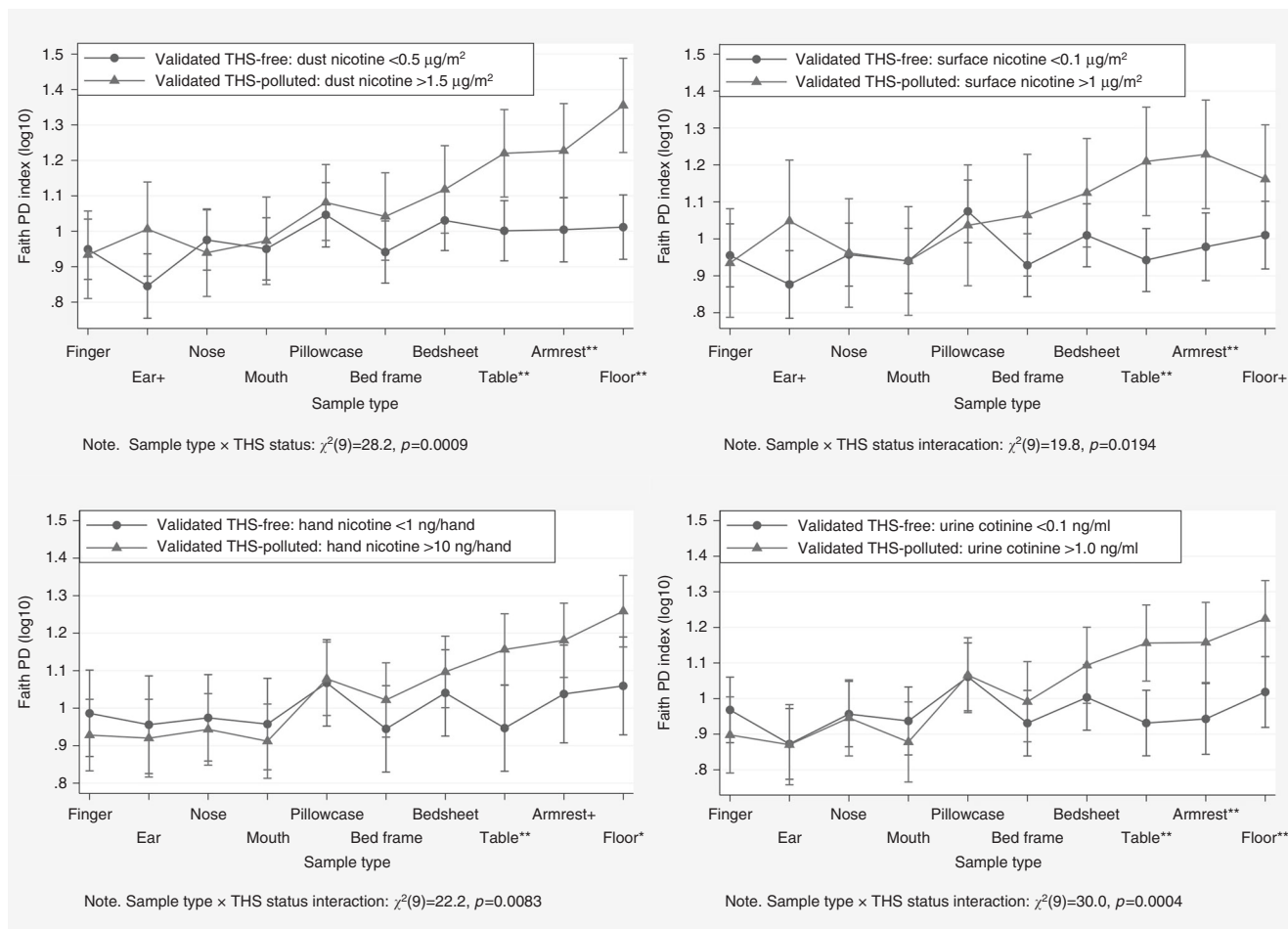
Fig. 2 Faith PD \alpha -diversity in human and environmental samples. The four panels show Faith PD means (in log0 scale) and their 95% confidence intervals of samples taken from validated THS-free (blue, vNEG) and THS-polluted (red, vTEG) homes based on dust nicotine, surface nicotine, hand nicotine, and urinary cotinine. Note: ^+p < 0.10 ; ^{**}p < 0.01 .
