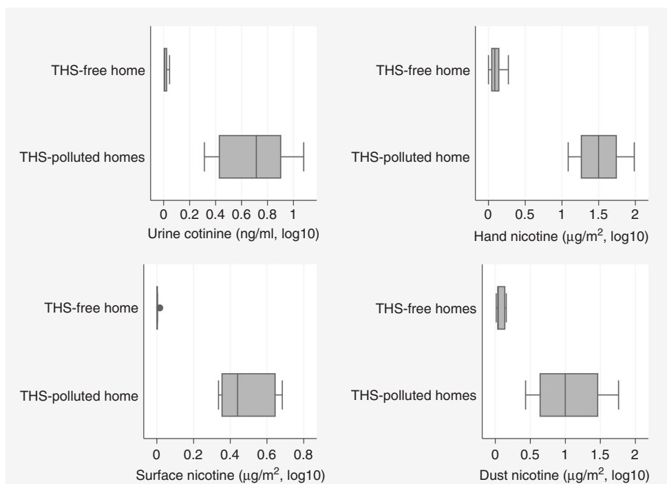
Fig. 1 Boxplots of THS pollution and exposure measures. The four panels show the distributions of urinary cotinine, hand nicotine, surface nicotine, and dust nicotine in the validated THS-free and THS-polluted homes.
