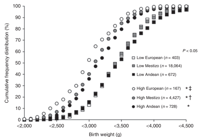
Figure 2. Cumulative frequency distribution. Values are the cumulative percentage of babies across weight intervals shown who were born at low or high altitude of Andean, Mestizo, or European ancestry. Significant differences ( P < 0.05 ) are as follows: *high vs. low; †Mestizo vs. Andean; ‡European vs. Mestizo or Andean (general linear model analysis of variance).
