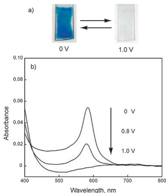
Figure 5. (a) Electrochromic behavior of FeL1-MEPE : a color of the polymer film changes from blue (left) to transparent/colorless (right) at 1.0 V vs. \text{Ag}/\text{Ag}^+ . (b) Electrochemical measurements of FeL1-MEPE film: UV-vis spectra of the polymer film at 0, 0.8, and 1.0 V vs. \text{Ag}/\text{Ag}^+ .
