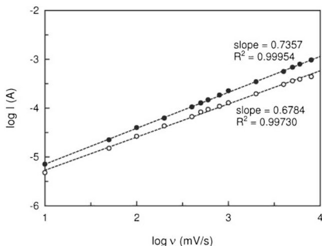
Figure 2. Scan rate dependencies of the peak current ( \log I_p - \log \nu ) for the cases of chloride- (○) and bromide-doped (●) polypyrrole films. The process of 'diffusion toward electrode surfaces' was provided by the \text{Fe}(\text{CN})_6^{3-}/\text{Fe}(\text{CN})_6^{4-} redox system. The peak currents recorded correspond to the oxidation of \text{Fe}(\text{CN})_6^{4-} ions.
