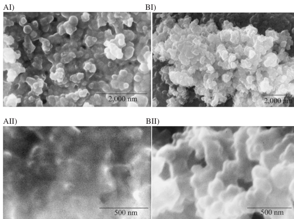
Figure 1. SEM images of (A) chloride- and (B) bromide-doped polypyrrole films electrodeposited onto Pt substrate surface.
