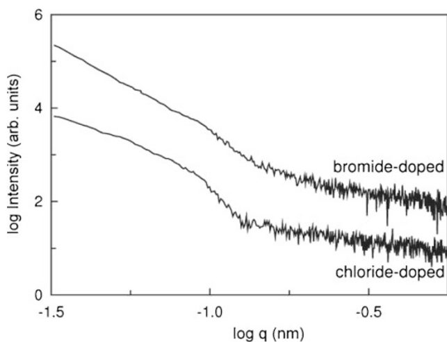
Figure 3. SAXS patterns reproduced in a logarithmic scale with respect to the q factor.
