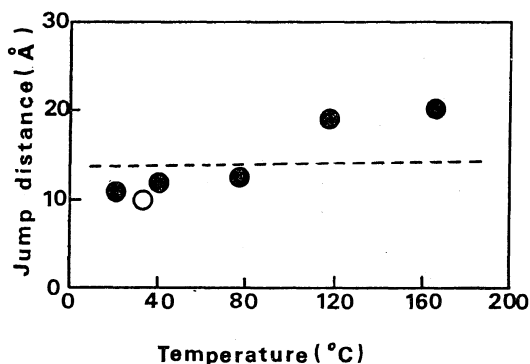
Figure 7. Jump distance vs. temperature: ●, jump distance; ○, mean free path of phonon; dotted line, diameter of monomer unit.
