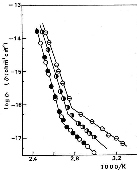
Figure 1. Electrical conductivity vs. reciprocal absolute temperature: ○, 0.014 MV/cm; ●, 0.086 MV/cm; ⊙, 0.36 MV/cm; ⊖, 0.74 MV/cm.
