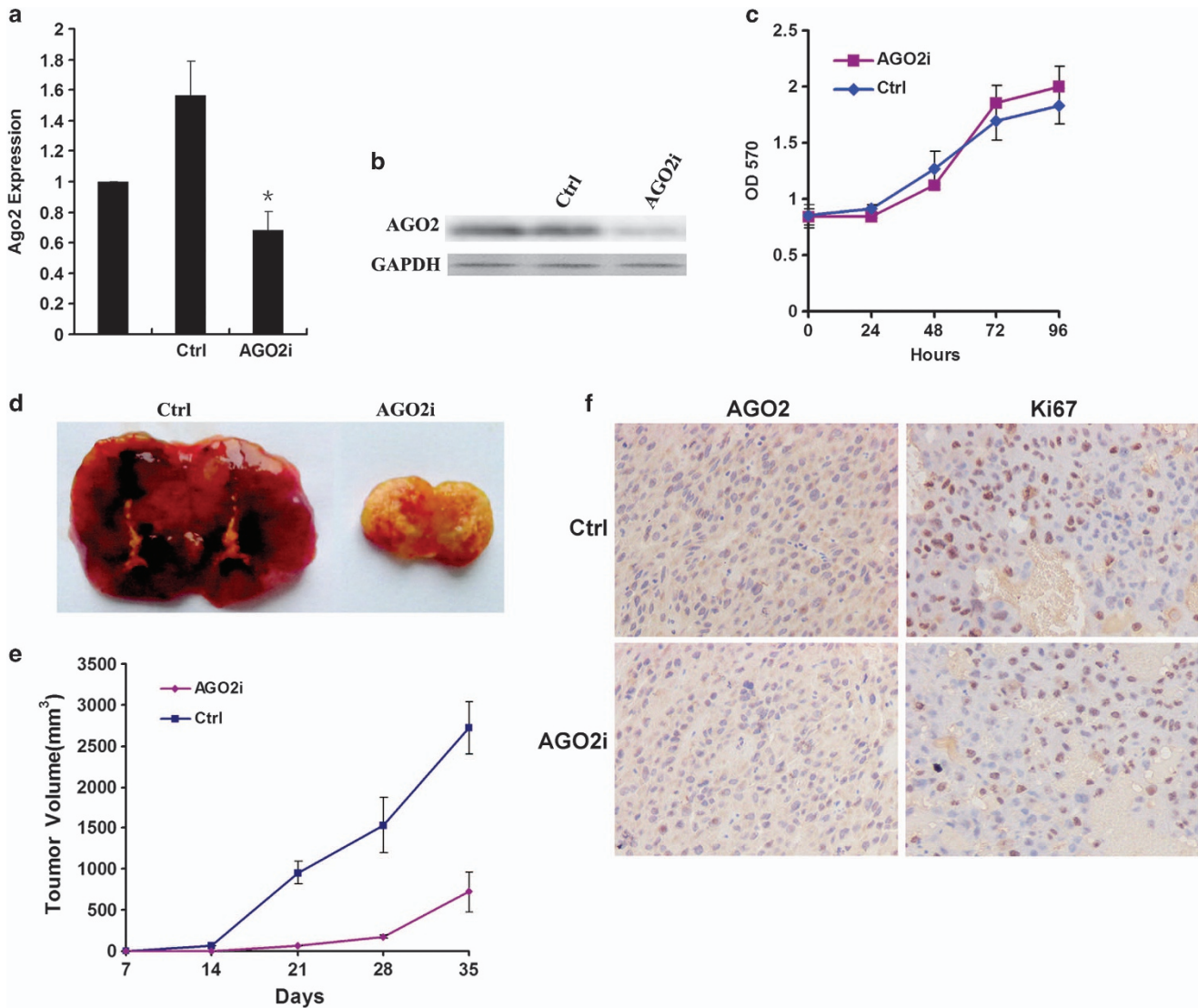
Figure 5. Ago2 knockdown distinctly inhibits HCC tumor growth in vivo . ( a, b ) Downregulation of Ago2 through lentivirus-mediated RNA interference (RNAi) as detected by RT-PCR and western blot. Ctrl and AGO2i indicated Huh7 cells stably expressing control siRNA and Ago2 -specific siRNA, respectively. ( c ) The effect on cell proliferation of Ago2 -knockdown as measured by MTT assay. Data were obtained from three independent experiments and shown as mean \pm s.d. ( d, e ) The influence on tumor growth by Ago2 knockdown in vivo . The growth curve and tumor morphology of Ago2 -knockdown Huh7 xenograft. ( f ) AGO2 and Ki67 expression examined by immunohistochemistry ( \times 200 ). Ctrl and AGO2i indicated Huh7 cells stably expressing control siRNA and Ago2 -specific siRNA, respectively.
