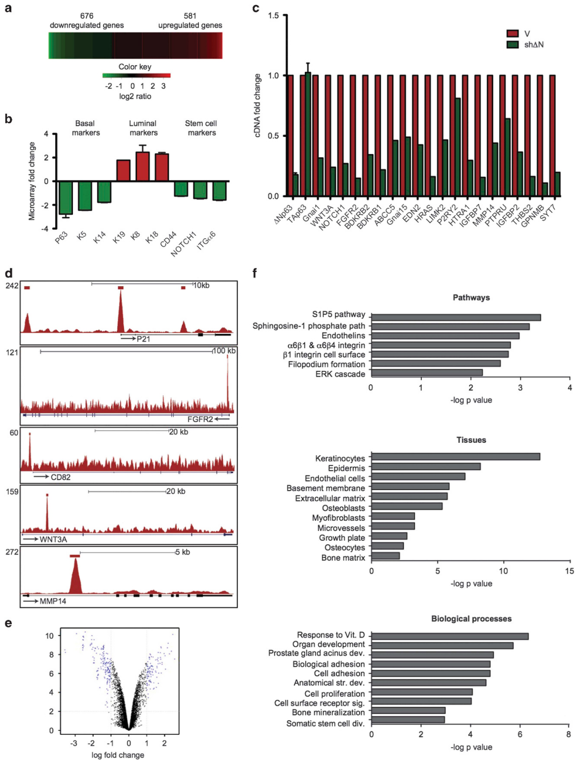
Figure 3. ΔNp63 directly regulates genes involved in epithelial development, stem cells and the bone microenvironment. (a) Microarray analysis of RWPE-1 cells infected with a short hairpin for ΔNp63 (R-shΔN) compared to RWPE-1 infected with vector control (R-V) was performed. The heat map represents the microarray results, with a fold change threshold of 1.4 and the P -value at 0.05. (b) Depiction of basal, luminal and stem cell genes that were up- and downregulated in R-shΔN, compared to R-V in the microarray. (c) RT-qPCR validation of some of the genes identified in the microarray. cDNA fold changes are compared to values in R-V. Two biological replicates are presented for ΔNp63 and TAp63, and one for the other genes. (d) ChIP-Seq analysis for p63 was performed in RWPE-1. Mapping peaks of p63 targets p21, FGFR2, WNT3A, BDKRB1 and MMP14 are shown. (e) Volcano plot of the common genes found in the microarray with ΔNp63 knockdown and ChIP-Seq. (f) Genomatix software analysis of direct p63-target genes downregulated in microarrays of R-shΔN compared to R-V showing the over-represented pathways, tissues and biological processes (full analysis and gene lists in Supplementary Table 2).
