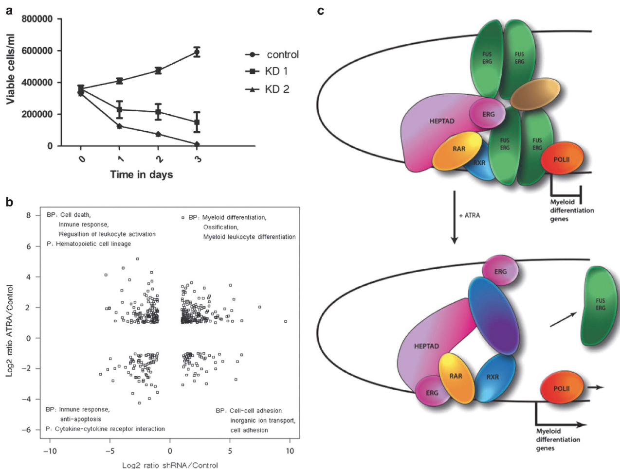
Figure 7. FUS-ERG knockdown alters the t(16;21) AML gene expression program. (a) Viability curves in TSU-1621-MT cells in samples with 23% knockdown (KD1) or 40% knockdown (KD2) of FUS-ERG over a period of 3 days. (b) Scatter plot of RPKM values (log 2 ) for FUS-ERG-regulated genes. The y axis represents expression of ATRA-treated genes versus control; the x axis represents expression of genes when induced with shRNA versus not induced. Each quadrant shows the gene enrichment for biological processes (BPs) and pathways (Ps). (c) Schematic model for the suggested actions of FUS-ERG in t(16;21) cells before and after ATRA treatment. Before treatment, FUS-ERG binds as an oligomer to promoter and intergenic regions together with a heptad of transcription factors, as well as RARA:RXR and RNAPII. After ATRA treatment, FUS-ERG is lost from the complex allowing RNAPII to transcribe genes involved in myeloid differentiation.
