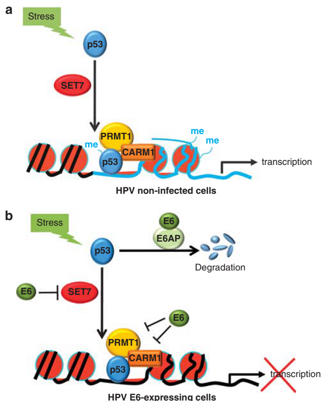
Figure 8 A model: E6 downregulates p53 function through HMT repression. (a) Previous reports indicate that, in HPV-non-infected cells, DNA-damage stress induces SET7-mediated p53 methylation and stabilization, as well as recruitment of p53 and its coactivators CARM1 and PRMT1 to p53-regulated genes for gene activation. (b) We demonstrate that, in HPV E6-expressing cells, in addition to directly targeting p53 for degradation through the E6AP pathway, E6 is able to inhibit SET7-mediated p53 methylation and thus reduce p53 protein stability. E6 can also target chromatin-bound p53 and repress the activities of the p53 coactivators CARM1 and PRMT1, leading to reduction of local histone methylation, which, likely, in turn dissociates p53 from chromatin. p53-dependent gene transcription is thus downregulated.
