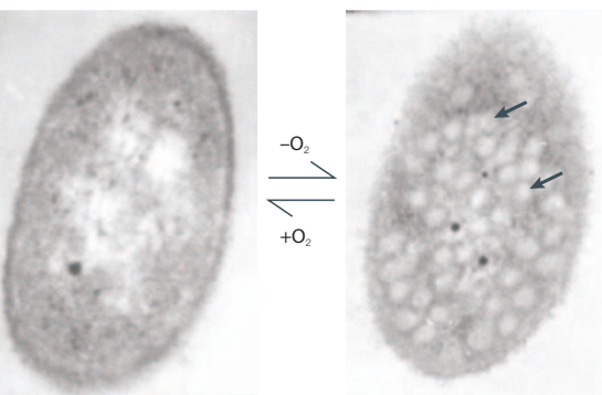
The transition of Rhodospirillum rubrum from an aerobic to anaerobic environment triggers regulatory events that result in the formation of photosynthetic membranes (indicated with arrows) under the regulatory control of PpsR, FnrL and PrrA. Image courtesy of C. Mackenzie, The University of Texas Health Science Center, USA.
