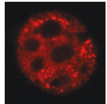
RNA fluorescence in situ hybridization showing the diffuse nuclear localization of CTN-RNA as well as its presence in paraspeckles in a mouse-embryo fibroblast. Image courtesy of Kannanganattu V. Prasanth and David L. Spector, Cold Spring Harbor Laboratory, USA.
