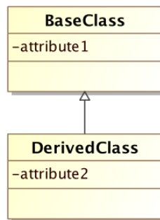
Figure 2.5: UML Generalisation
