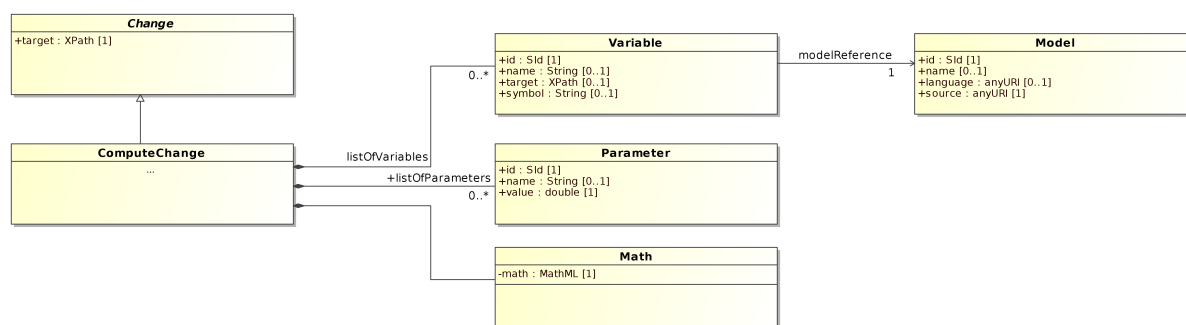
Figure 2.26: The ComputeChange class
