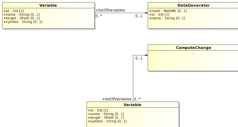
Figure 2.12: The SED-ML listOfVariables container
