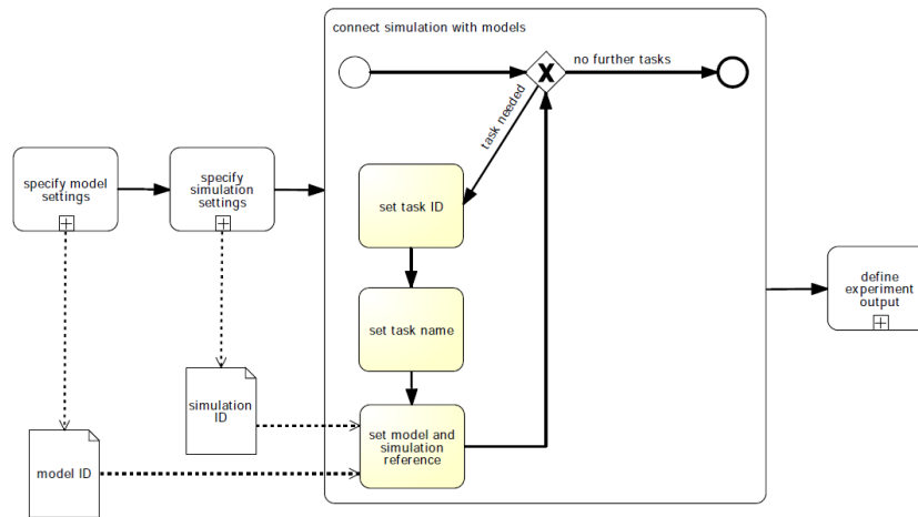
Figure 1.10: The process of defining simulation task(s) in SED-ML
