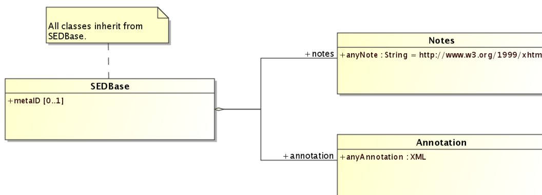
Figure 2.8: The SEDBase class
