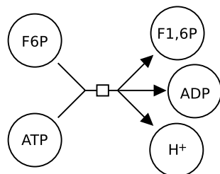
Figure 2.27: Reaction between ATP and fructose-6-phosphate to produce fructose-1,6-biphosphate, ADP and a proton.
