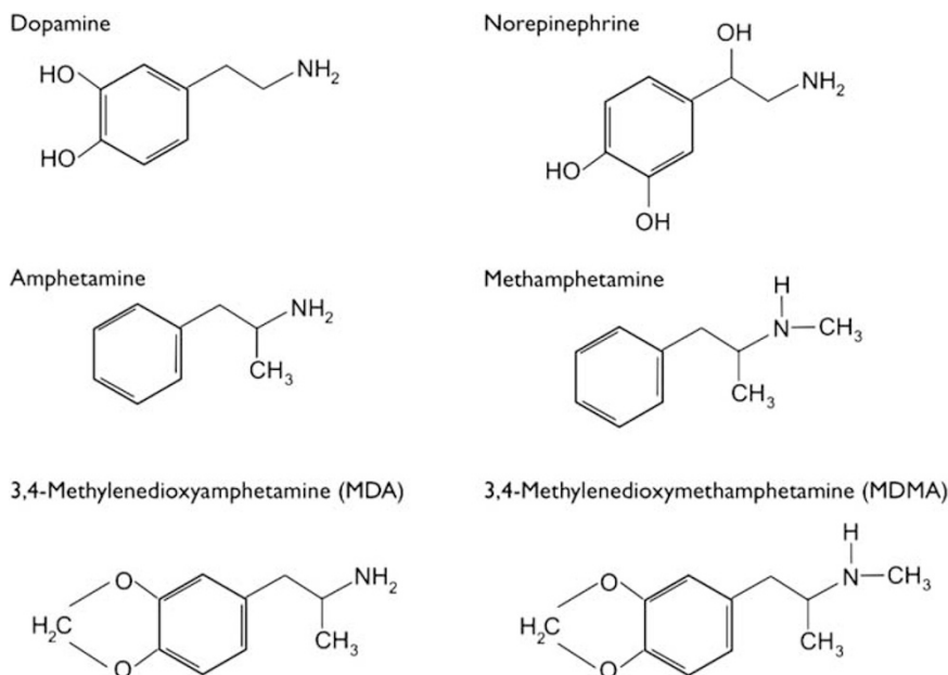
Figure 1 Chemical structure of neurotransmitters and amphetamines.
